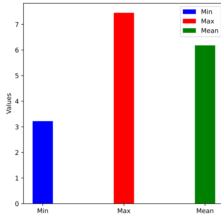
Resolvent Count
