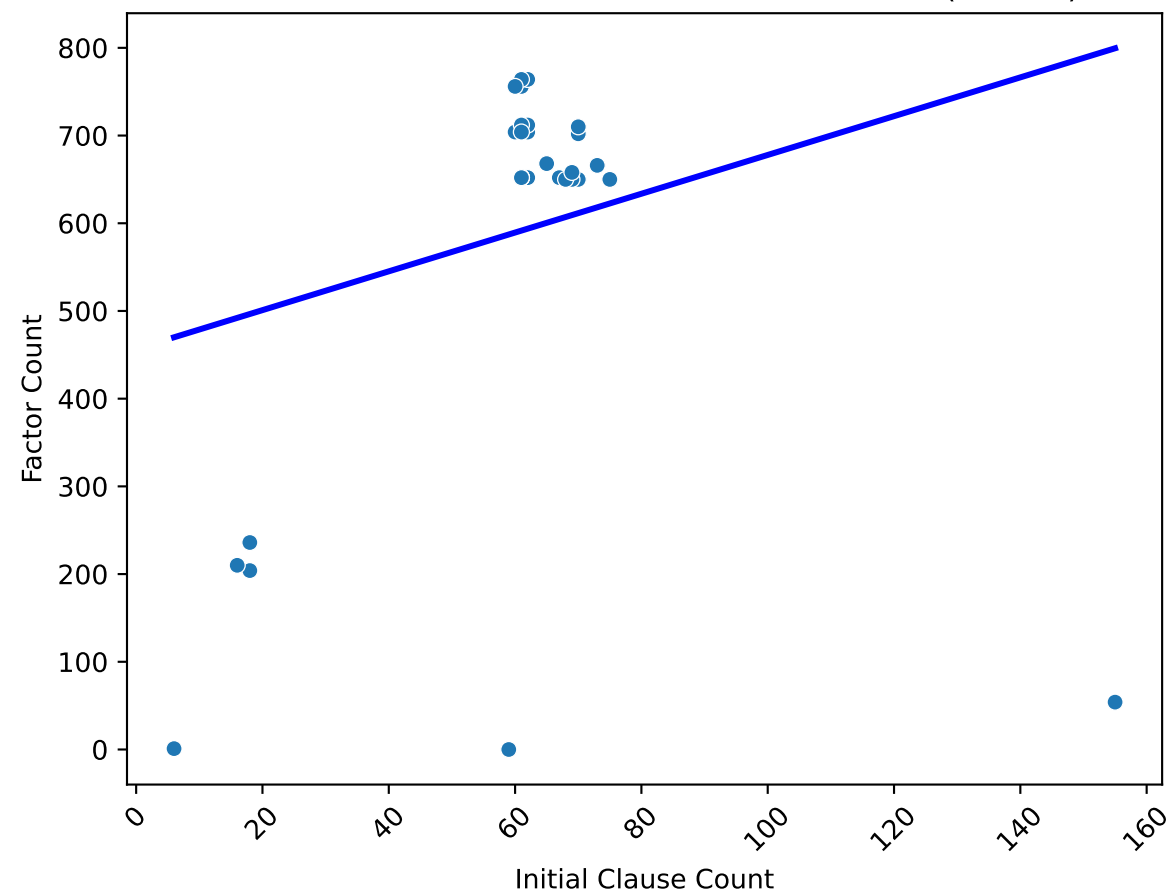
Correlation between Initial and Factor Counts ( r=0.23 )
