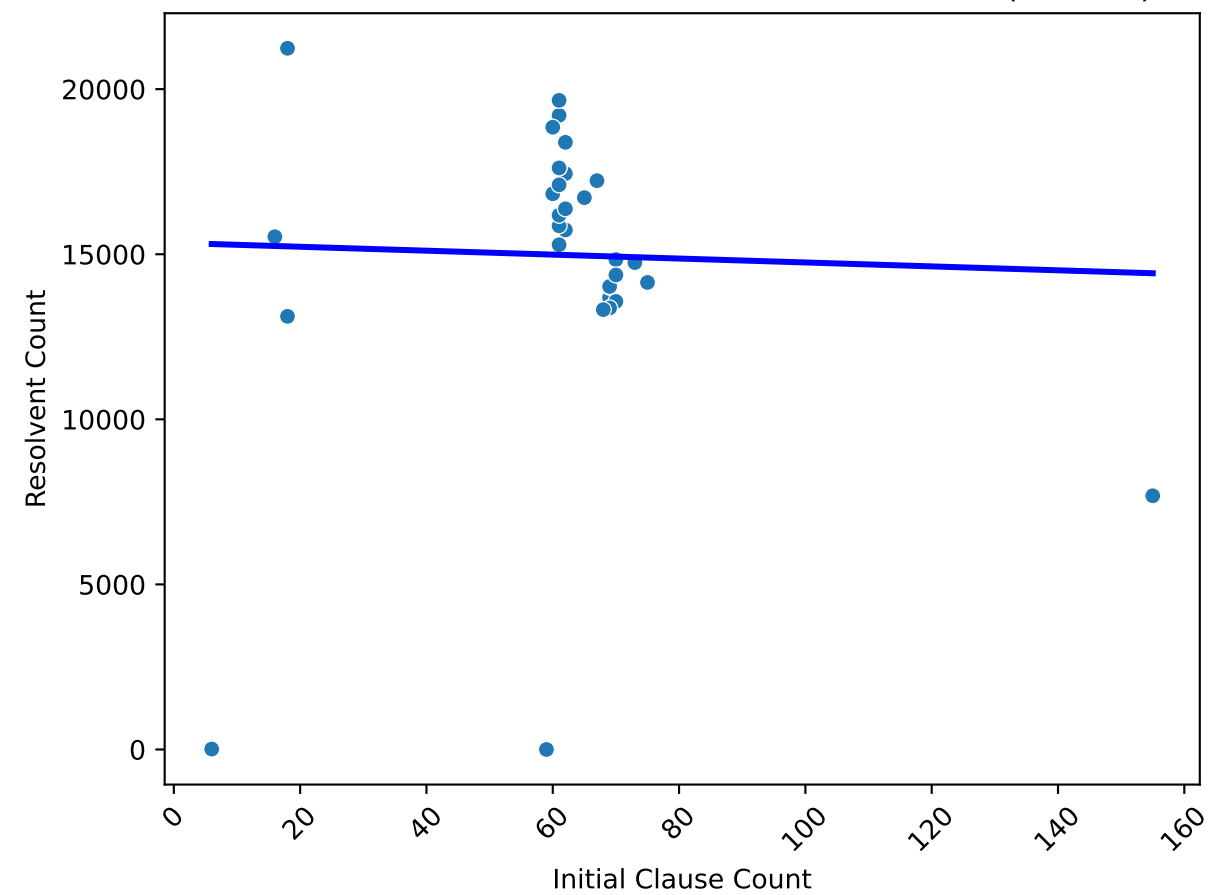
Correlation between Initial and Resolvent Counts ( r=-0.03 )
