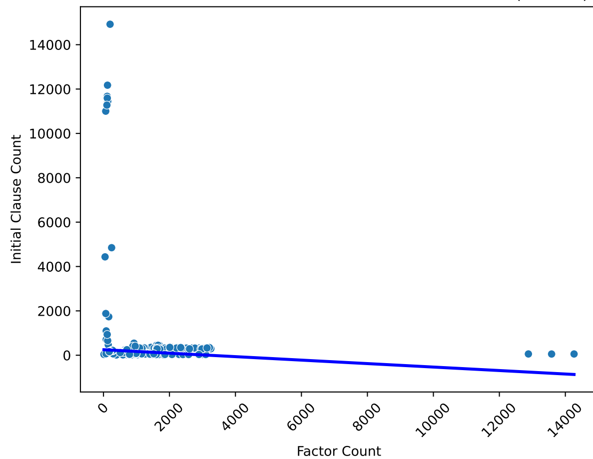
Correlation between Factor and Initial Clause Counts ( r=-0.07 )
