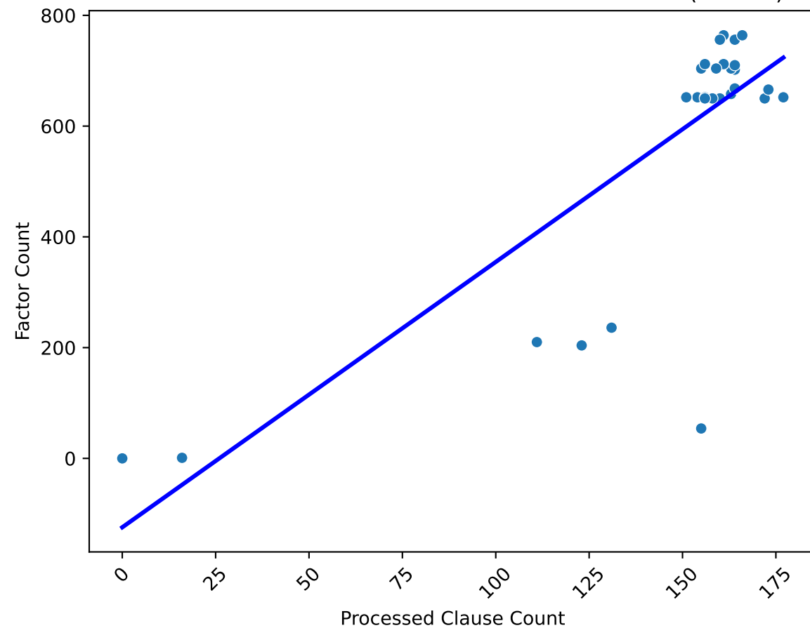
Correlation between Processed and Factor Counts ( r=0.80 )
