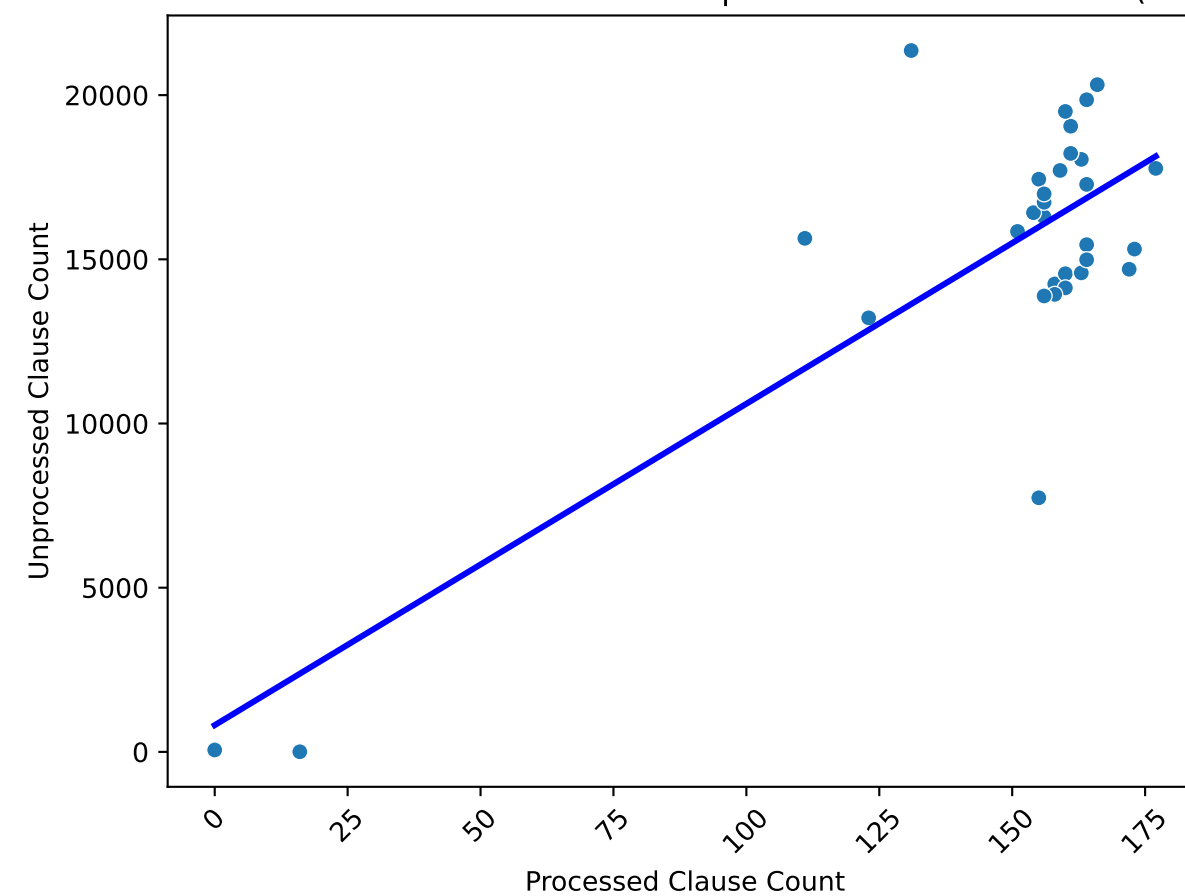
Correlation between Processed and Unprocessed Clause Counts ( r=0.80 )
