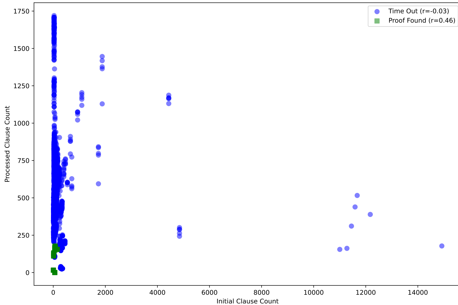
Correlation between Initial and Processed Clause Counts ( r=-0.03 )
