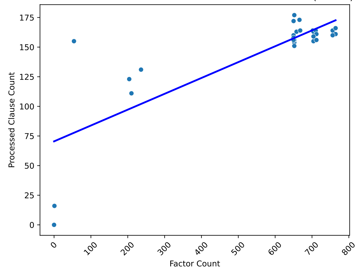
Correlation between Factor and Processed Clause Counts ( r=0.80 )
