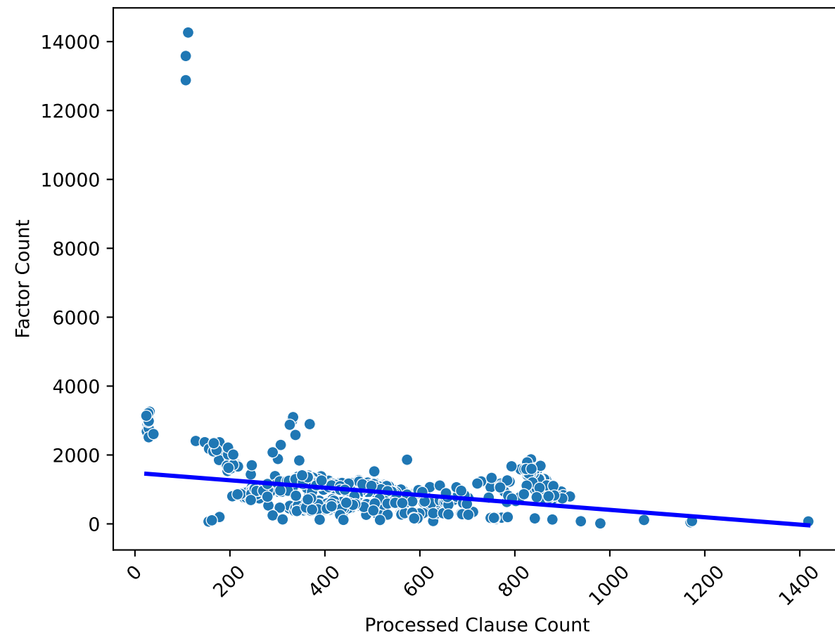
Correlation between Processed and Factor Counts ( r=-0.25 )
