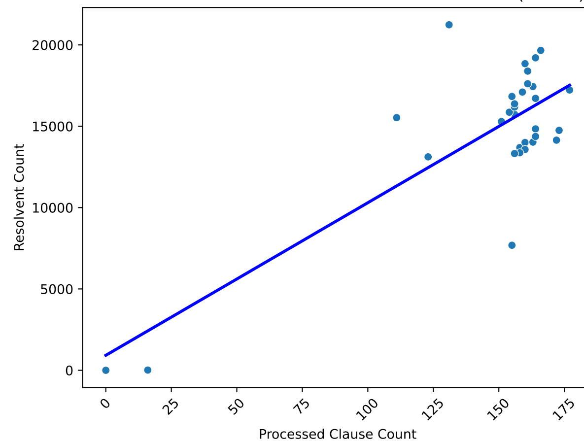
Correlation between Processed and Resolvent Counts ( r=0.79 )
