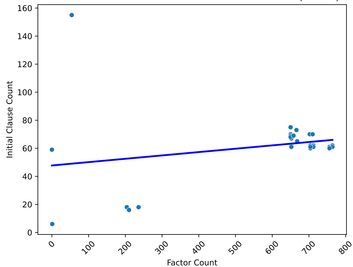
Correlation between Factor and Initial Clause Counts ( r=0.23 )
