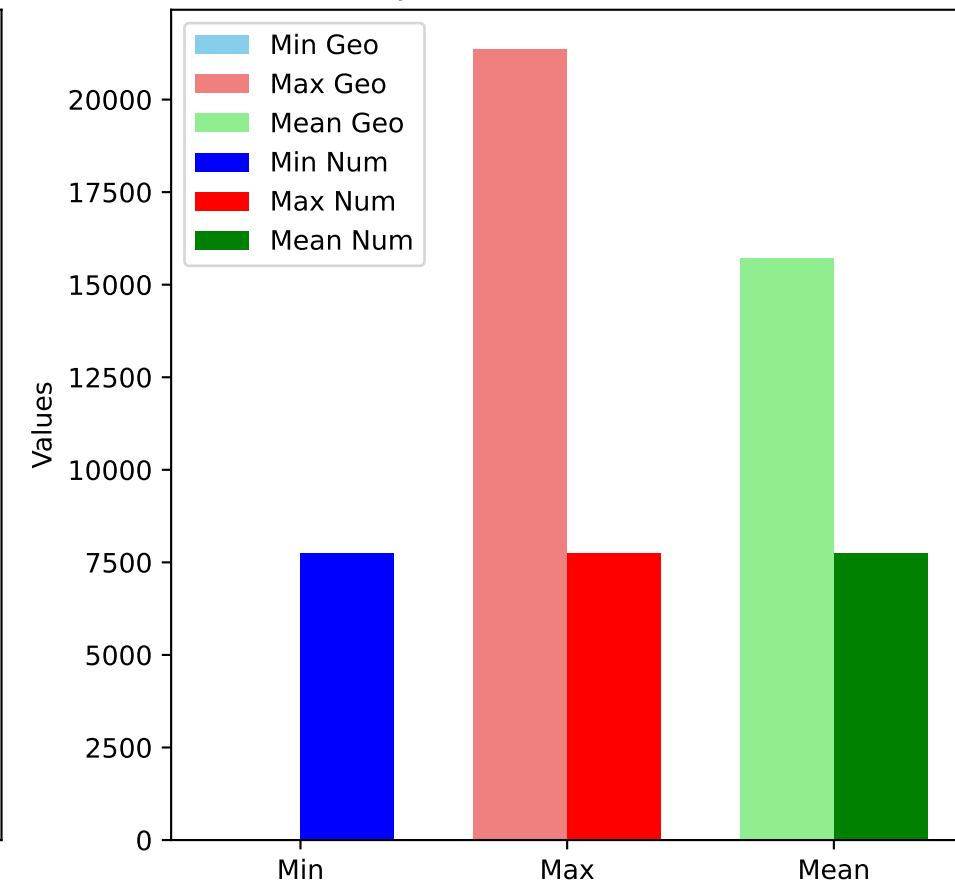
Unprocessed Clause Count
