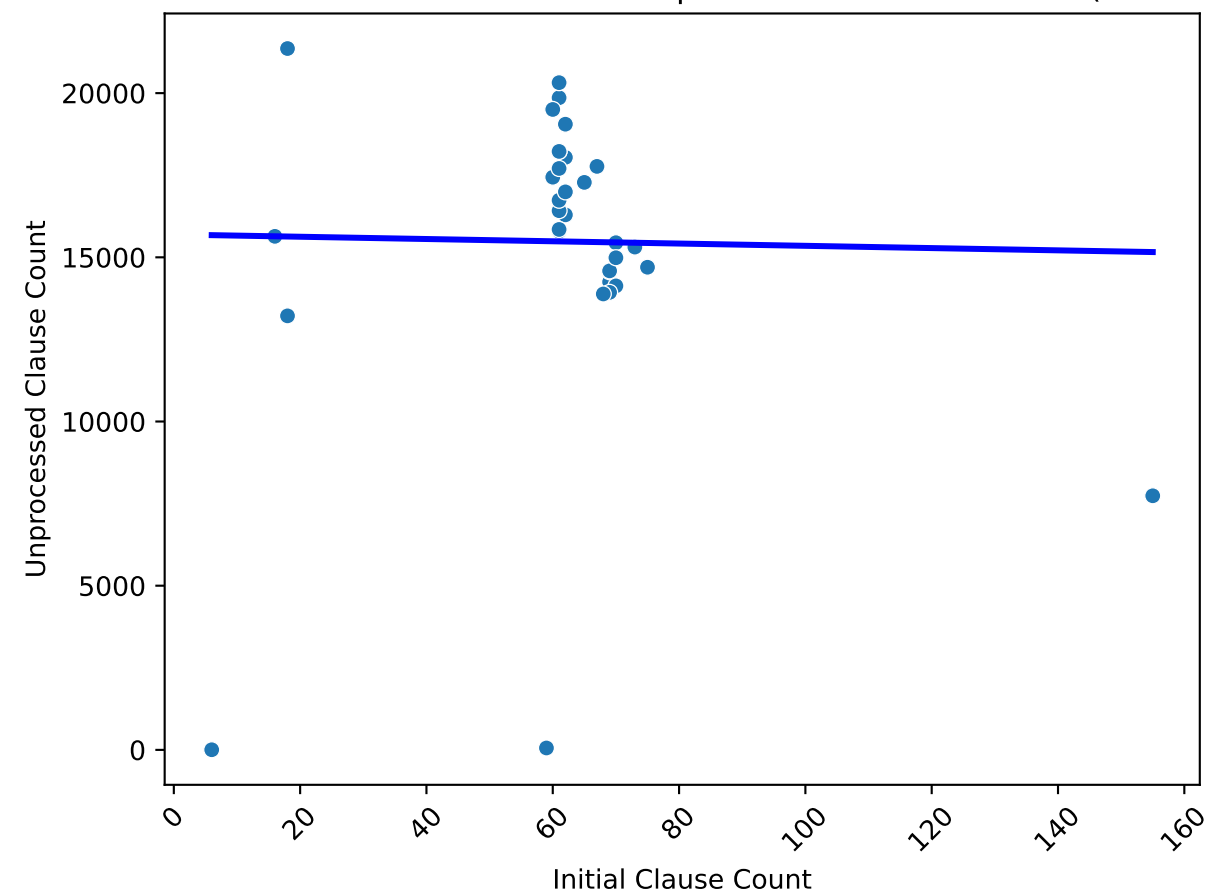
Correlation between Initial and Unprocessed Clause Counts ( r=-0.02 )
