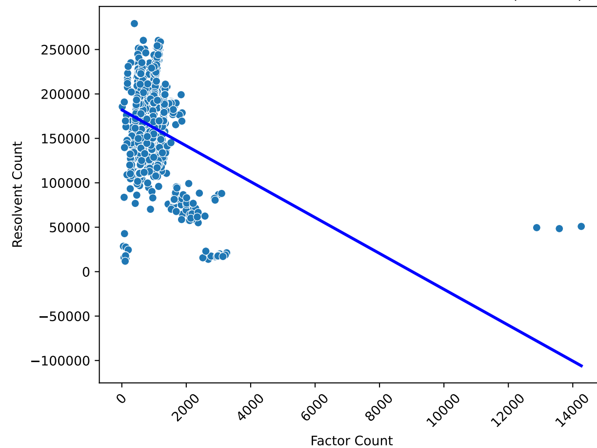
Correlation between Factor and Resolvent Counts ( r=-0.34 )
