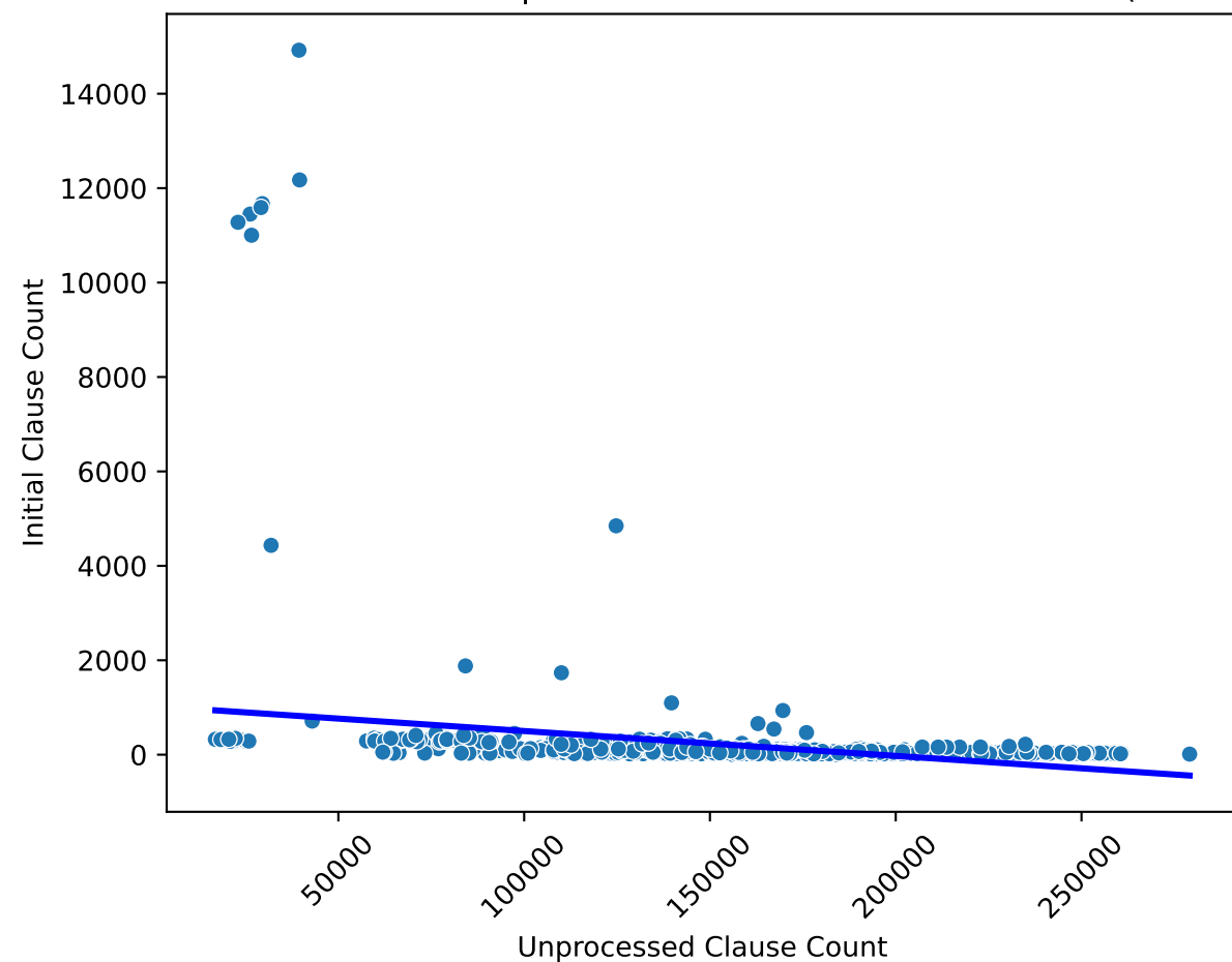
Correlation between Unprocessed and Initial Clause Counts ( r=-0.28 )
