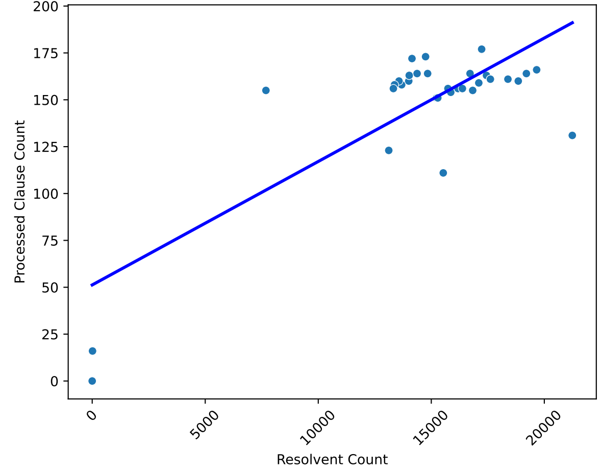
Correlation between Resolvent and Processed Clause Counts ( r=0.79 )
