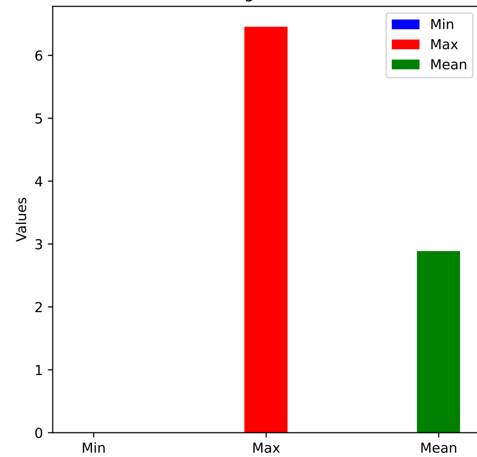
Tautologies Deleted
