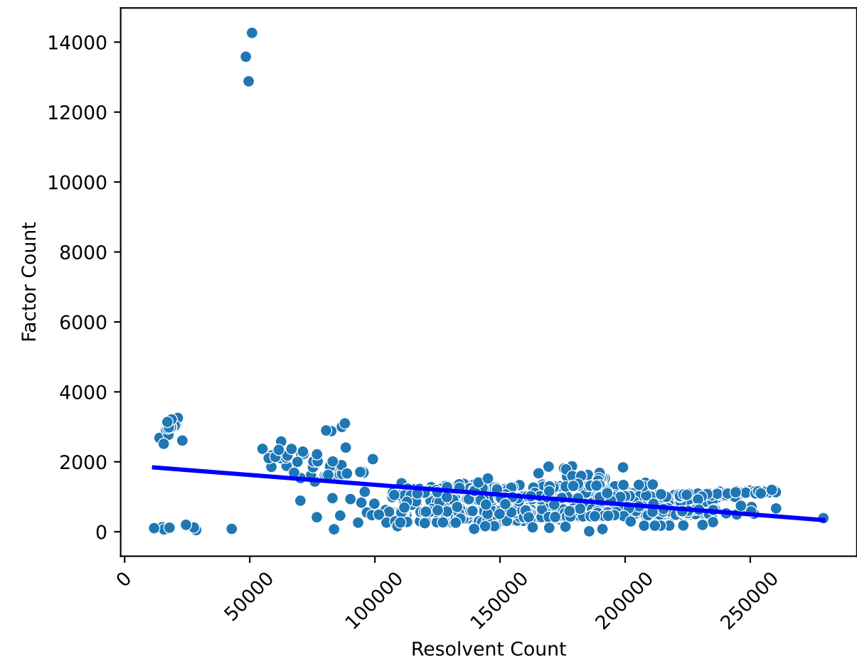
Correlation between Resolvent and Factor Counts ( r=-0.34 )
