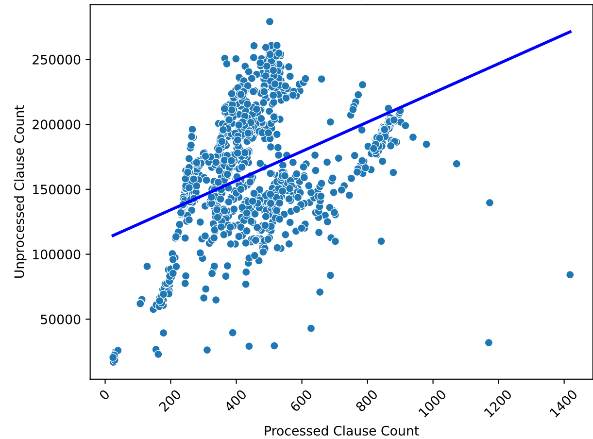
Correlation between Processed and Unprocessed Clause Counts ( r=0.44 )
