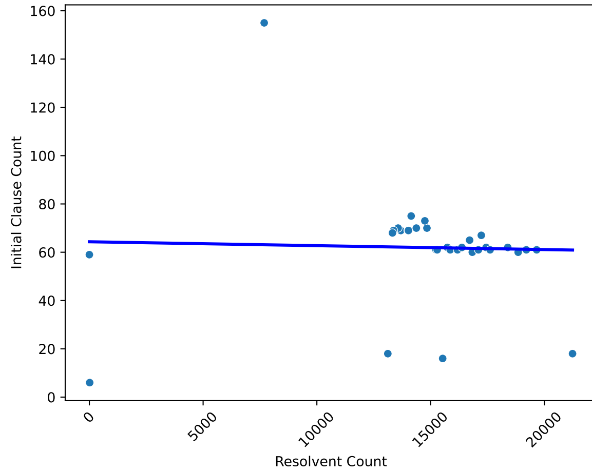
Correlation between Resolvent and Initial Clause Counts ( r=-0.03 )
