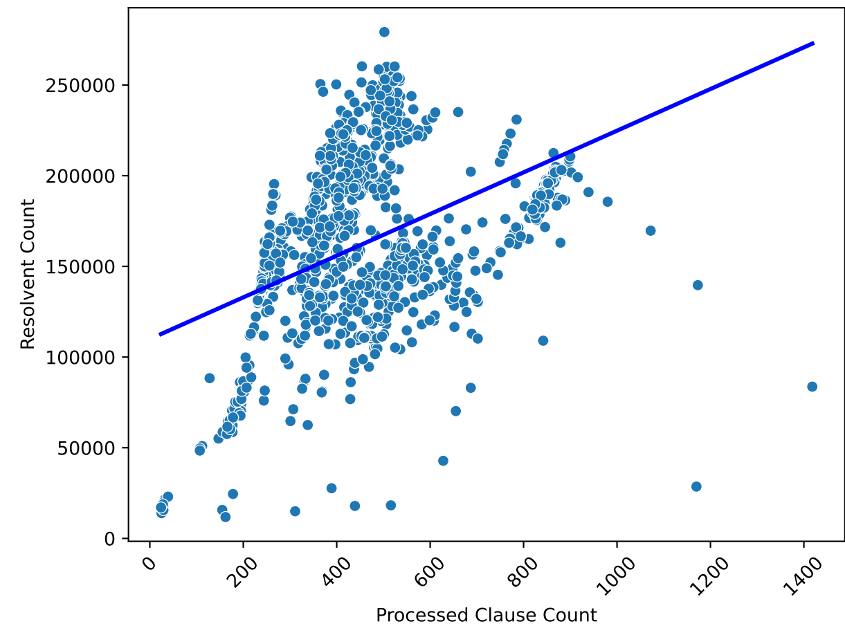
Correlation between Processed and Resolvent Counts ( r=0.44 )
