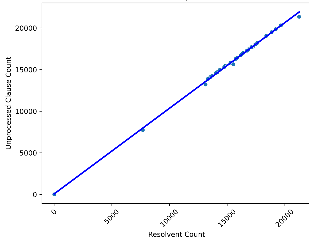
Correlation between Resolvent and Unprocessed Clause Counts ( r=1.00 )
