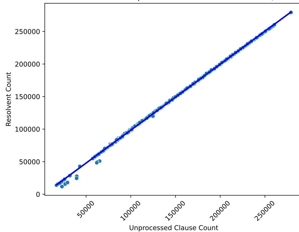
Correlation between Unprocessed and Resolvent Counts ( r=1.00 )
