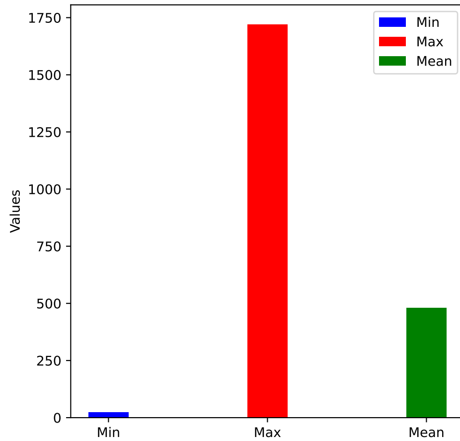
Resolvent Count
