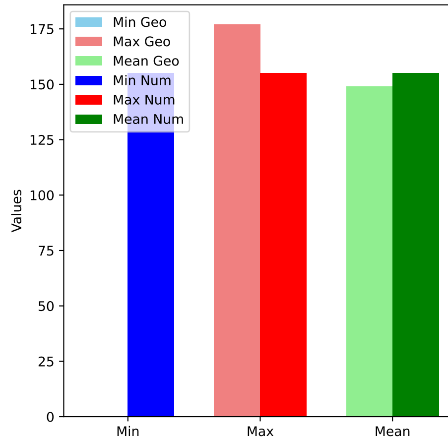
Resolvent Count
