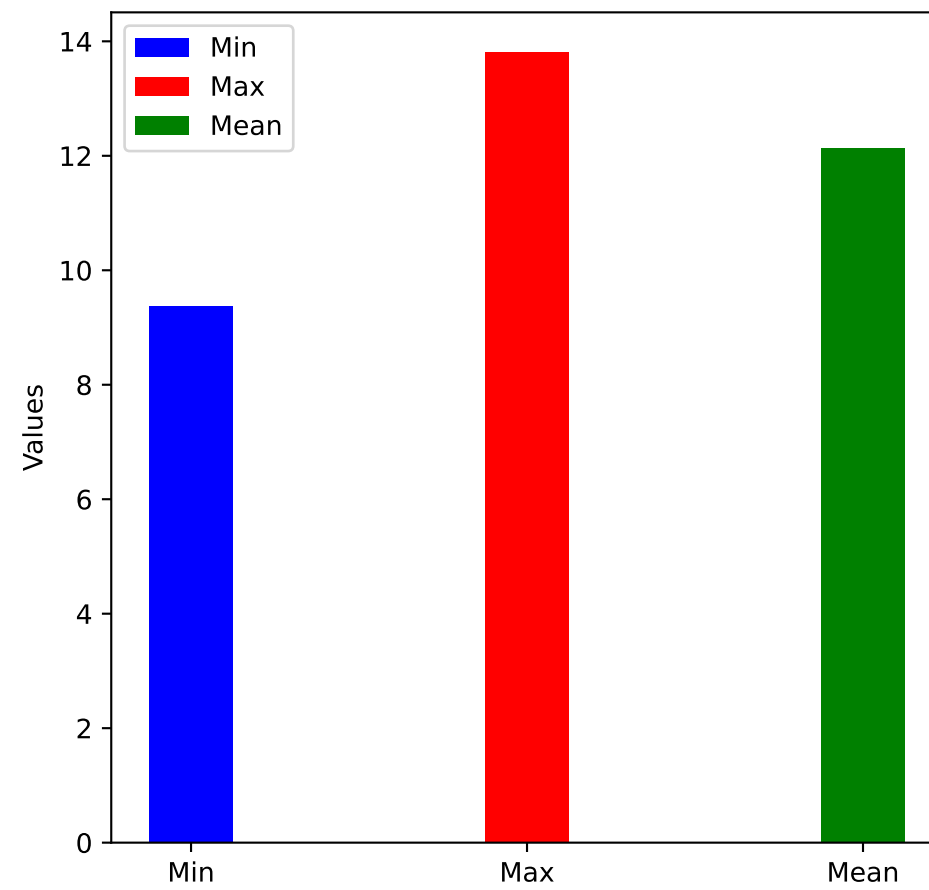
Resolvent Count
