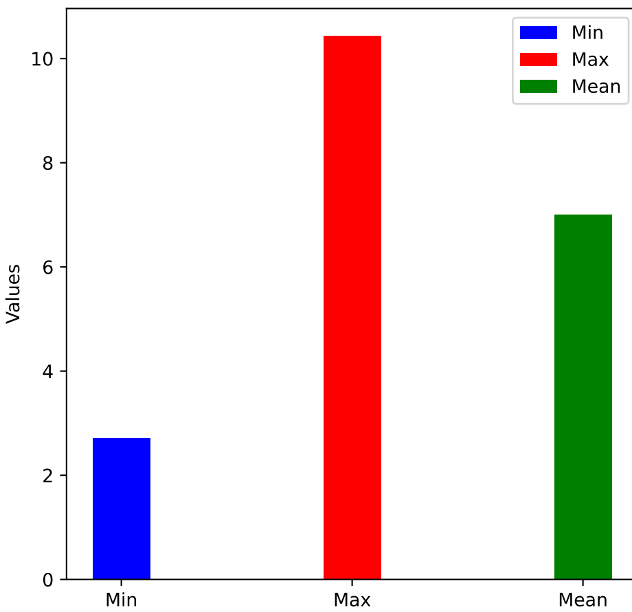
Factor Count
