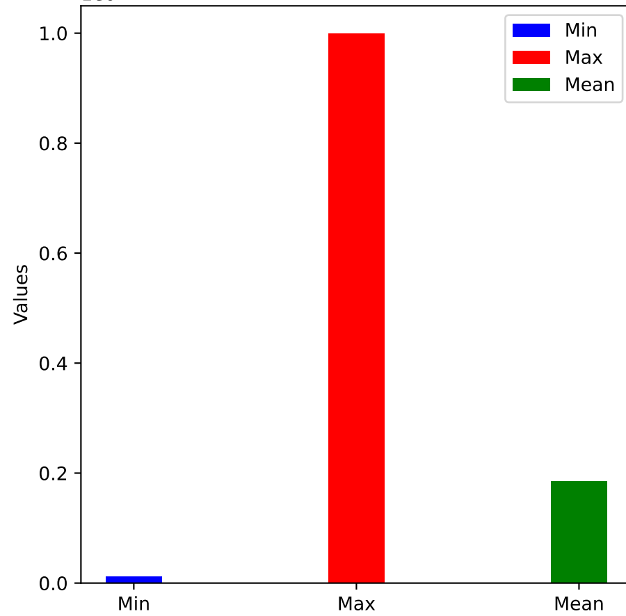
Resolvent Count
