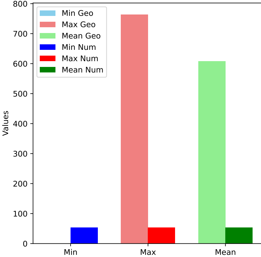
Factor Count
