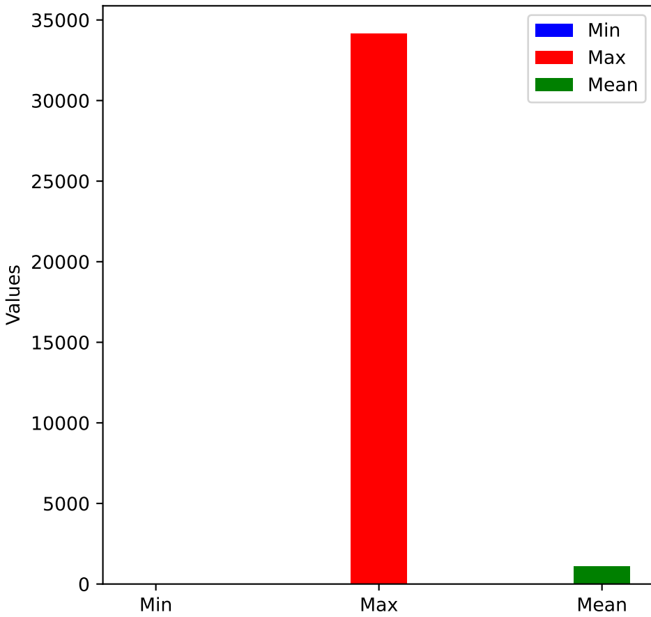
Factor Count
