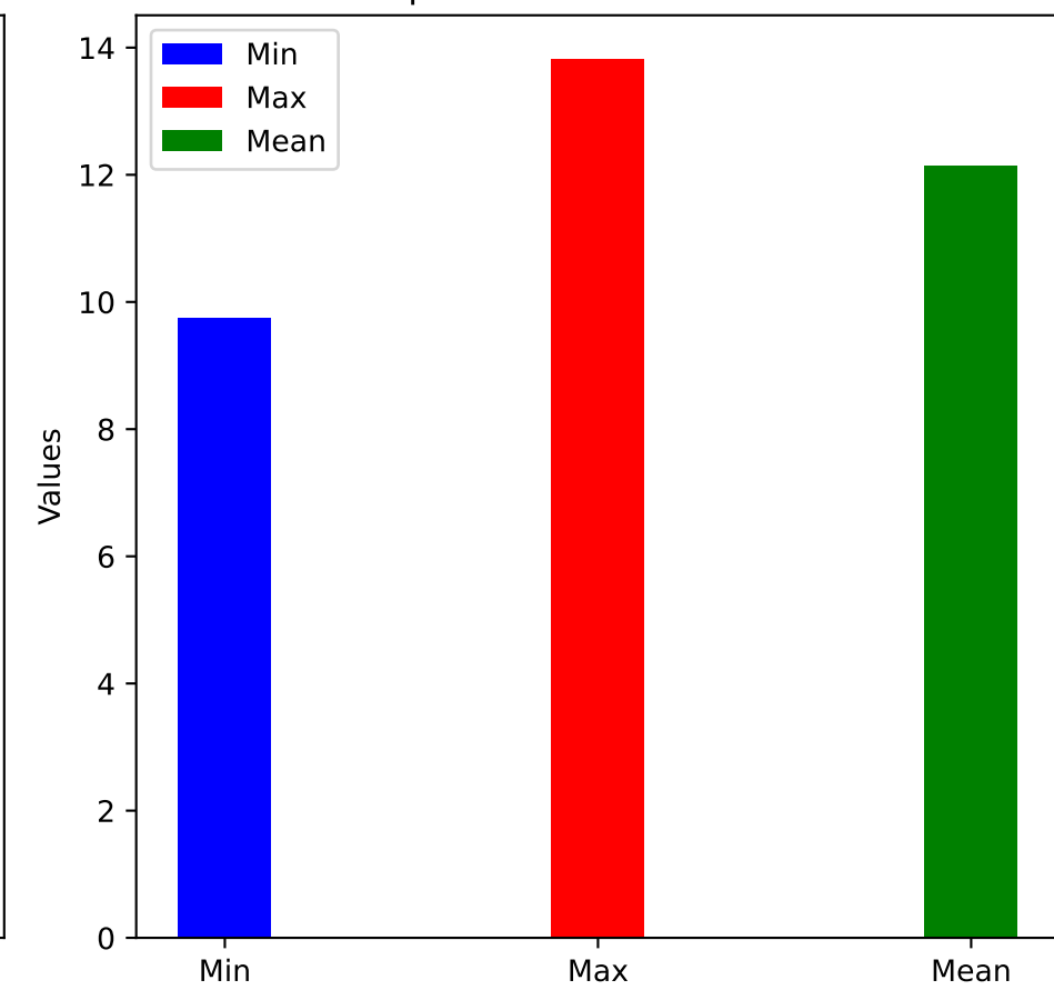
Tautologies Deleted
