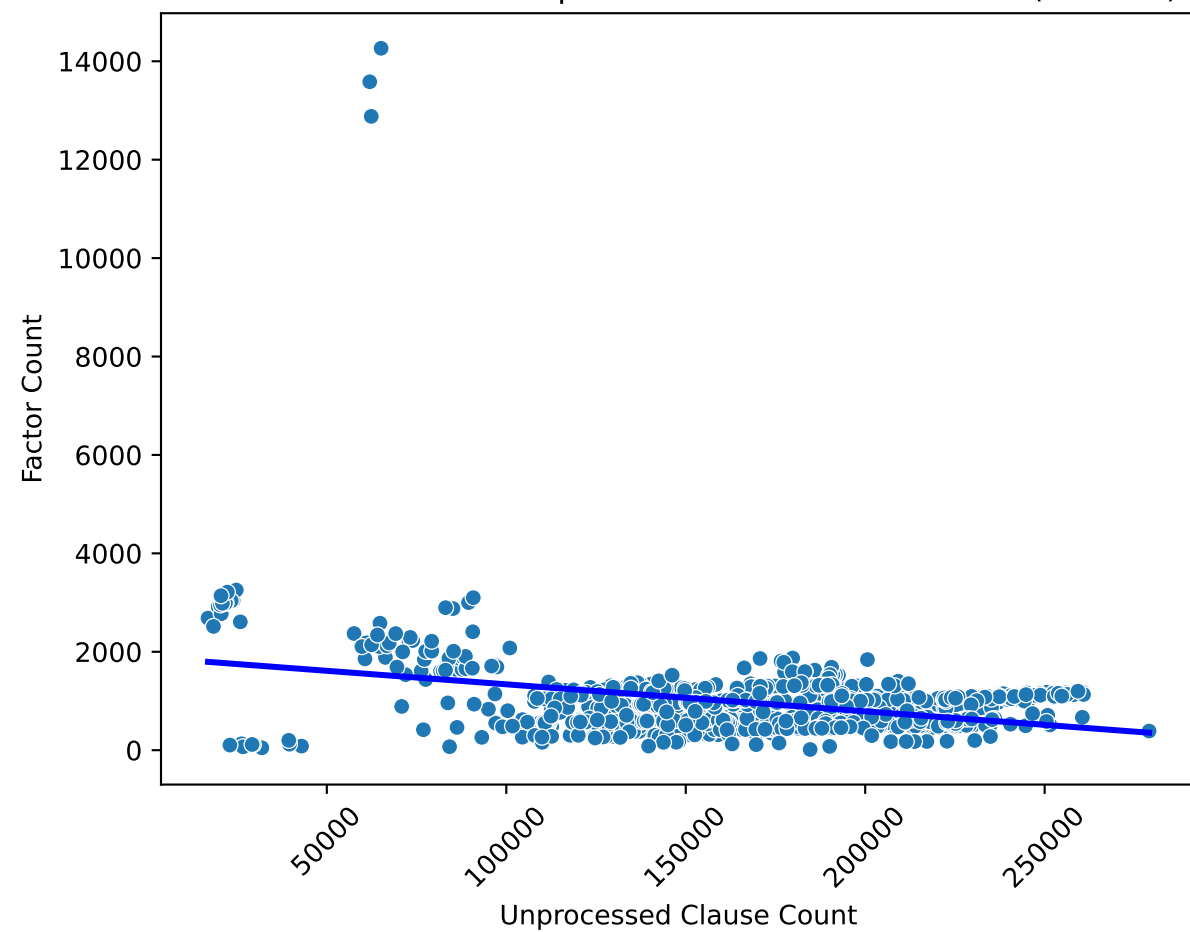
Correlation between Unprocessed and Factor Counts ( r=-0.32 )
