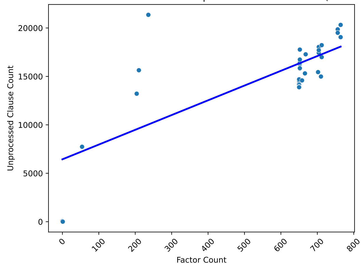
Correlation between Factor and Unprocessed Clause Counts ( r=0.74 )
