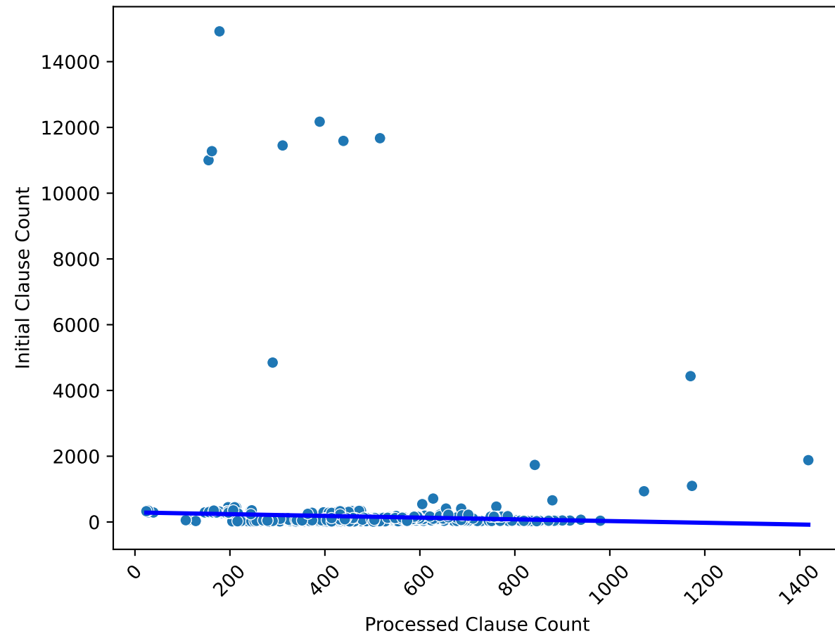
Correlation between Processed and Initial Clause Counts ( r=-0.05 )
