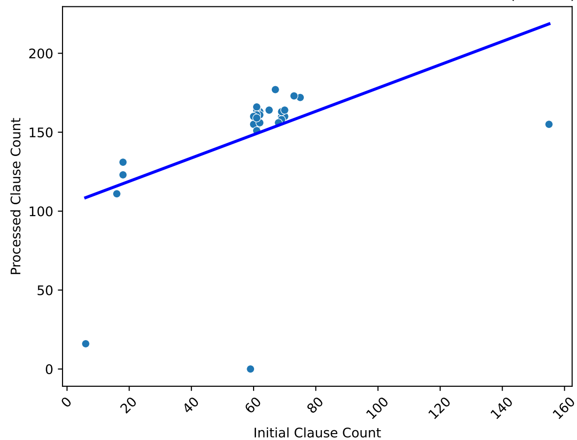
Correlation between Initial and Processed Clause Counts ( r=0.46 )
