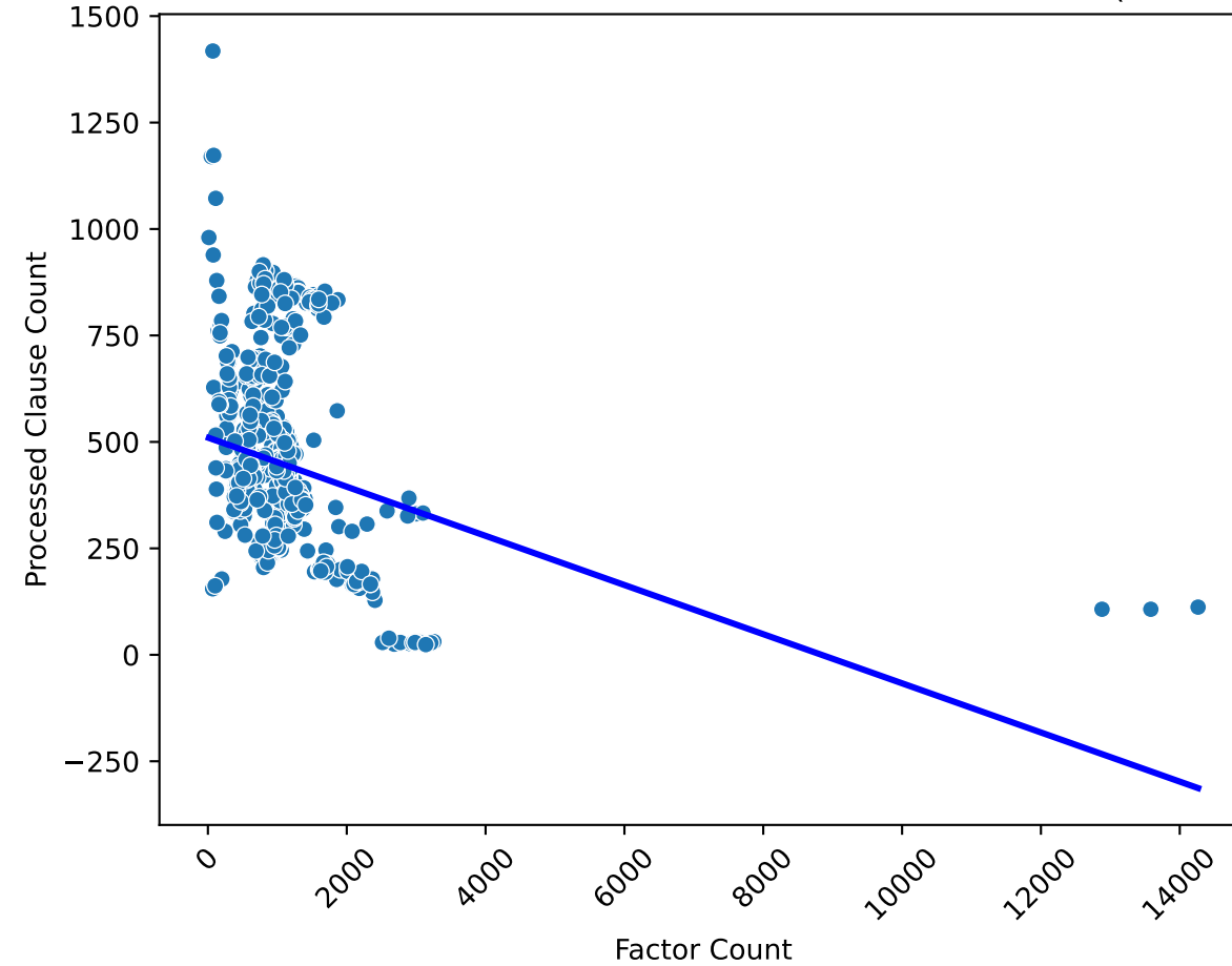
Correlation between Factor and Processed Clause Counts ( r=-0.25 )
