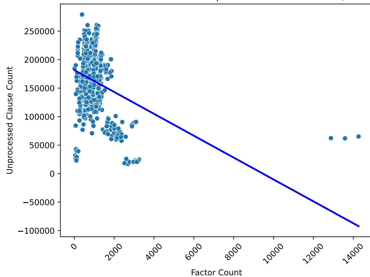
Correlation between Factor and Unprocessed Clause Counts ( r=-0.32 )
