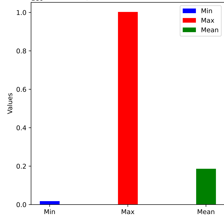
Tautologies Deleted
