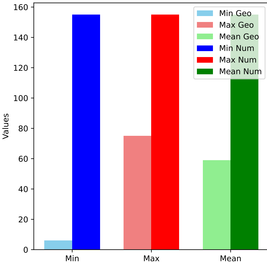
Factor Count
