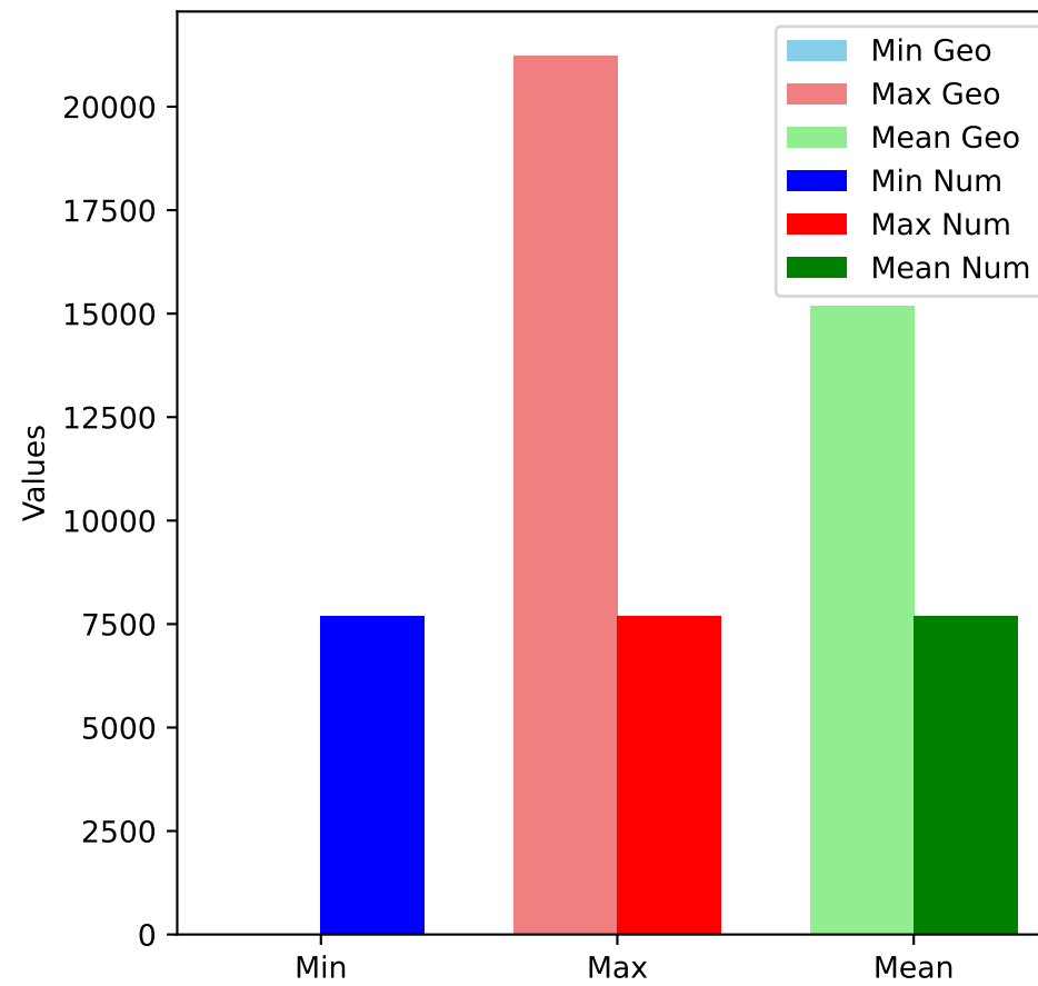
Resolvent Count
