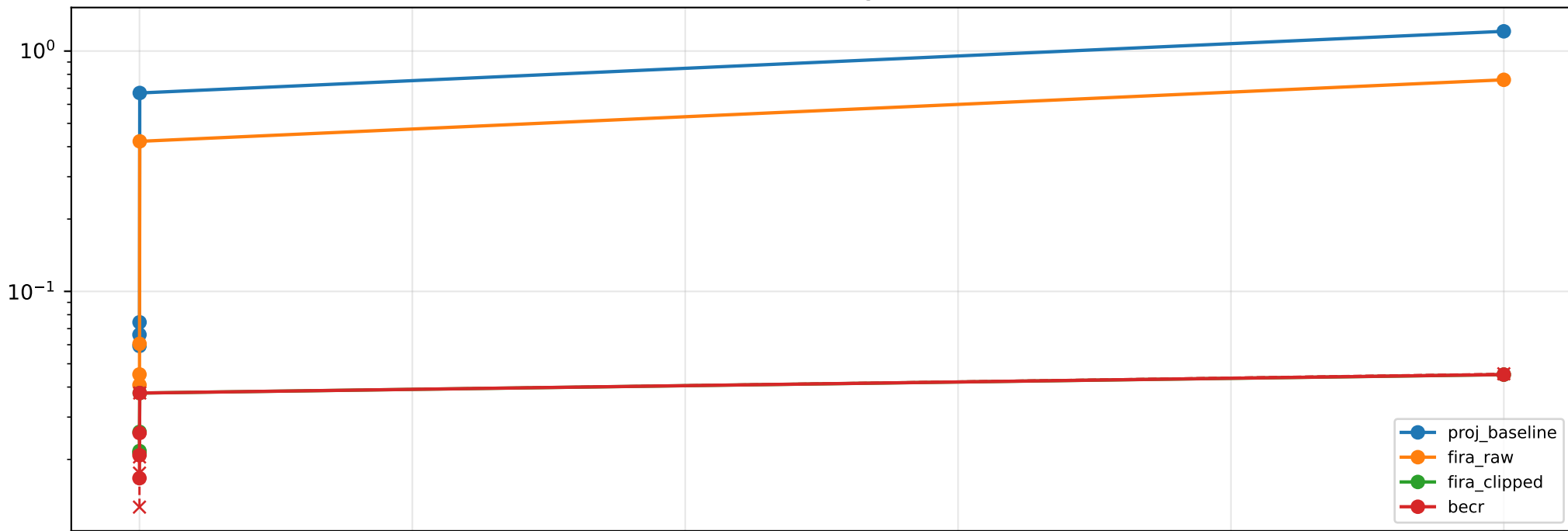
Coordinate diagnostics
