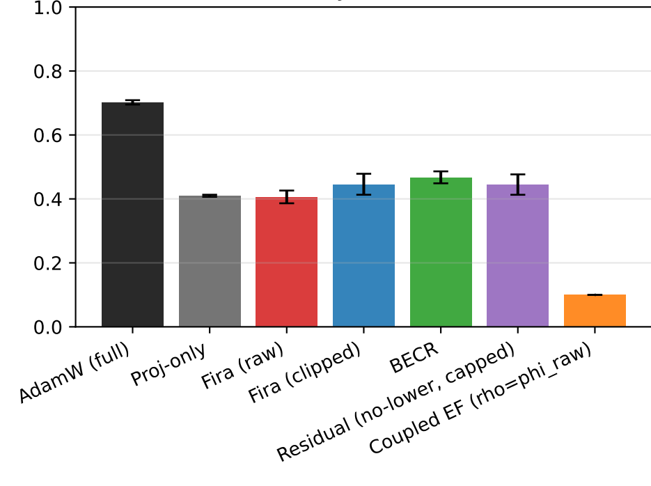
(f) Final test accuracy (mean \pm std over seeds)
