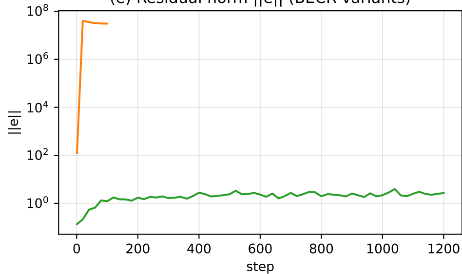
(e) Residual norm \|e\| (BECR variants)
