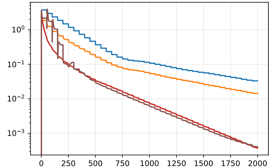
(f) f(x_t)
