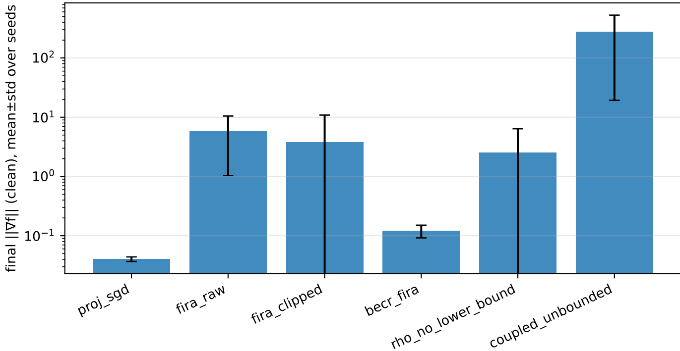
Exp3: anisotropic-noise + SVD-biased projection
