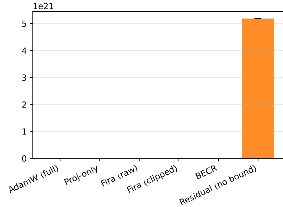
(f) Final valid perplexity (mean \pm std over seeds)
