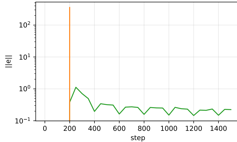
(e) Residual norm ||e|| (BECR variants)
