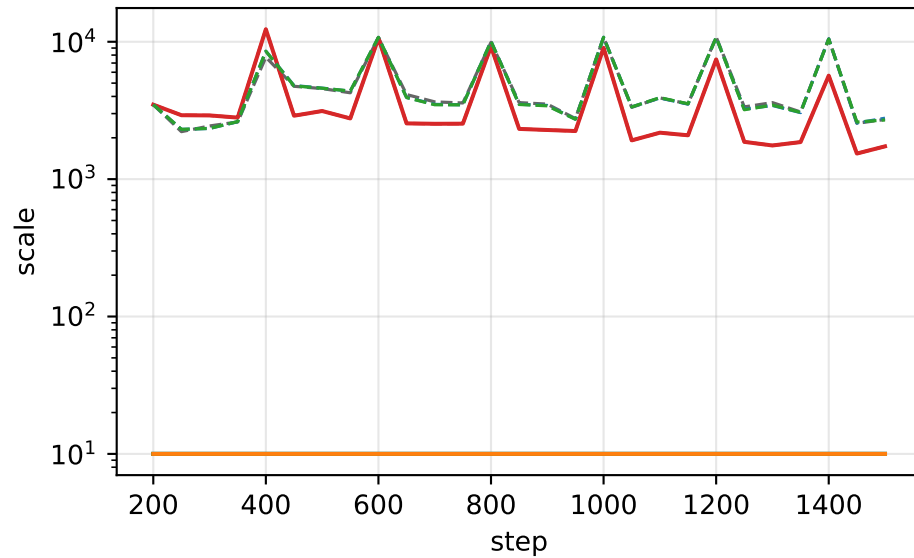
(d) Scale p95: s_t (solid) vs \phi_{\text{raw}} (dashed)
