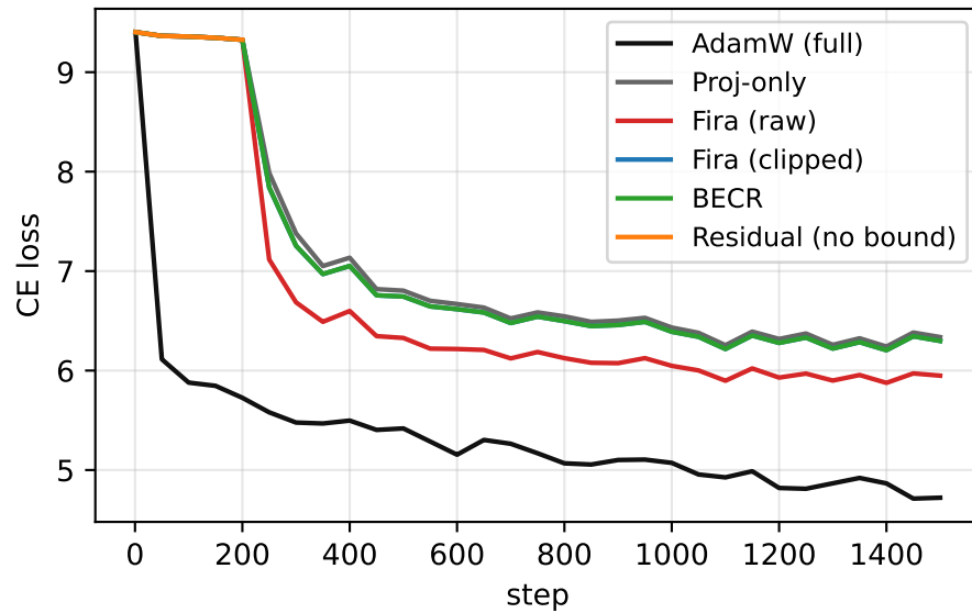
(a) Train loss (seed=0)
