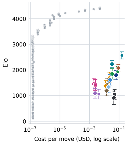
(a) KataGo and LLMs
