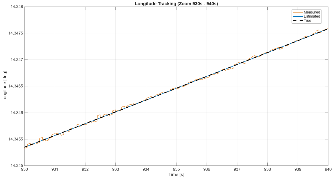
Figure 5.19: Longitude trajectory tracking (zoomed): Comparison between ground-truth, noisy GNSS measurement, and the ESKF estimation.
