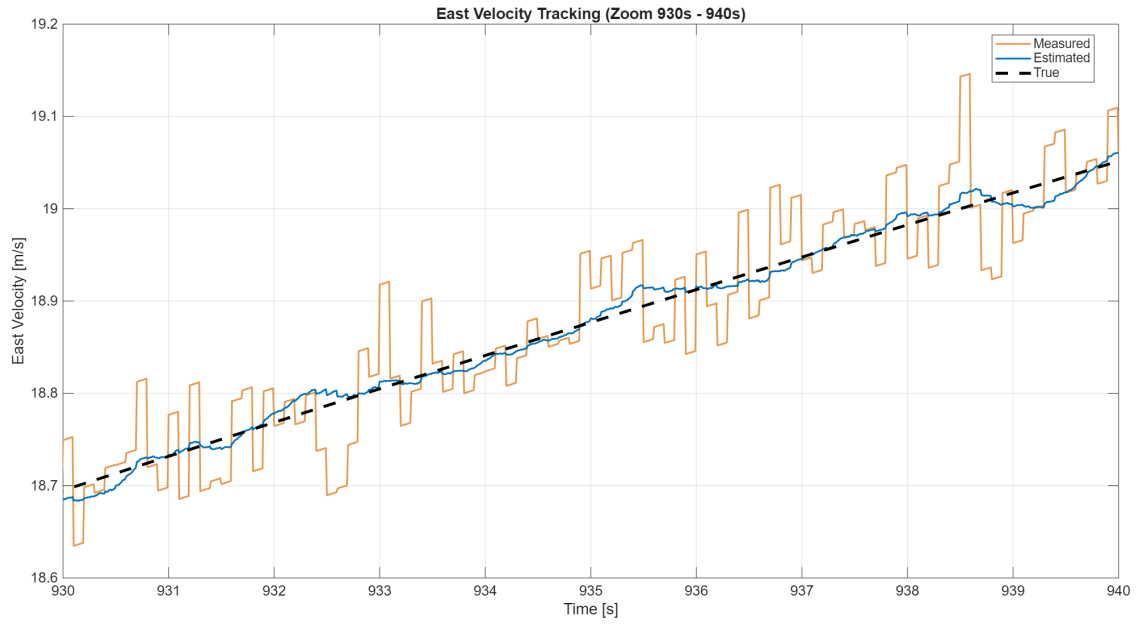
Figure 5.13: East velocity trajectory tracking (zoomed): Comparison between ground-truth, noisy GNSS measurement, and the ESKF estimation.
