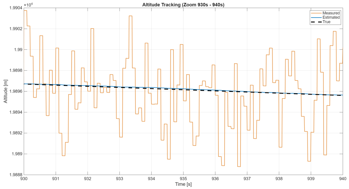
Figure 5.17: Altitude trajectory tracking (zoomed): Comparison between ground-truth, noisy GNSS measurement, and the ESKF estimation.
