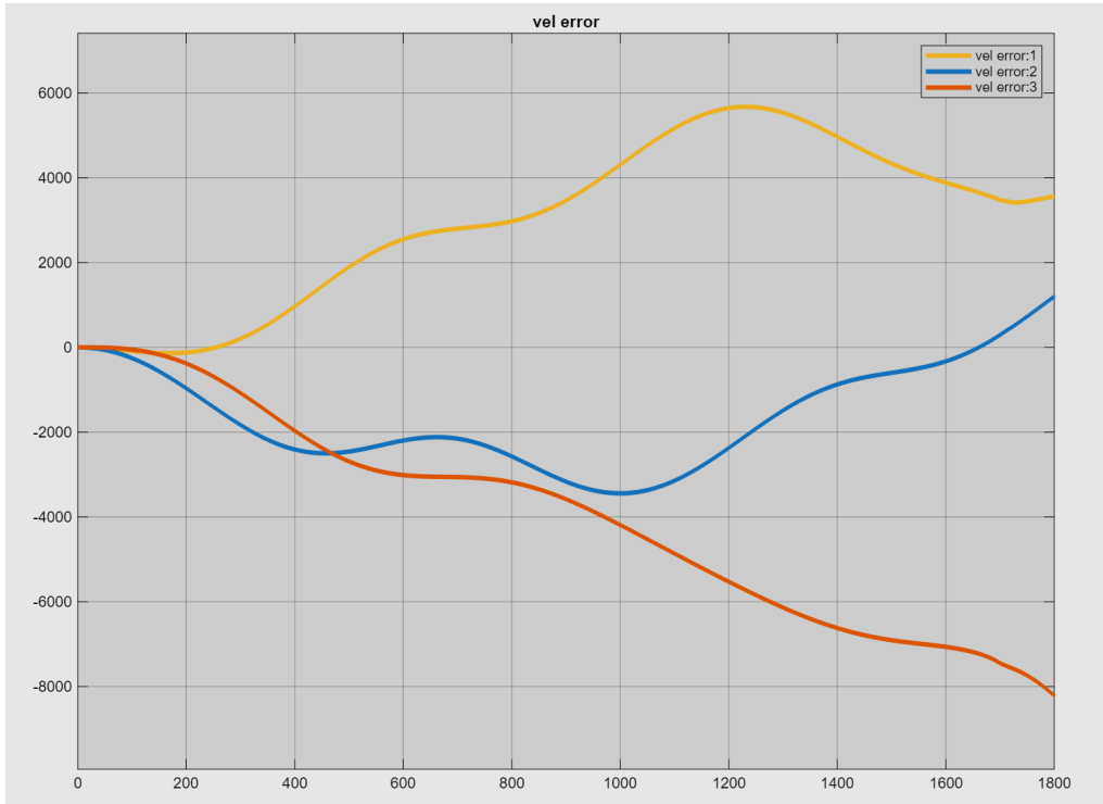
Figure 5.10: Time evolution of the velocity estimation error resulting from pure mechanization, with no filter applied.
