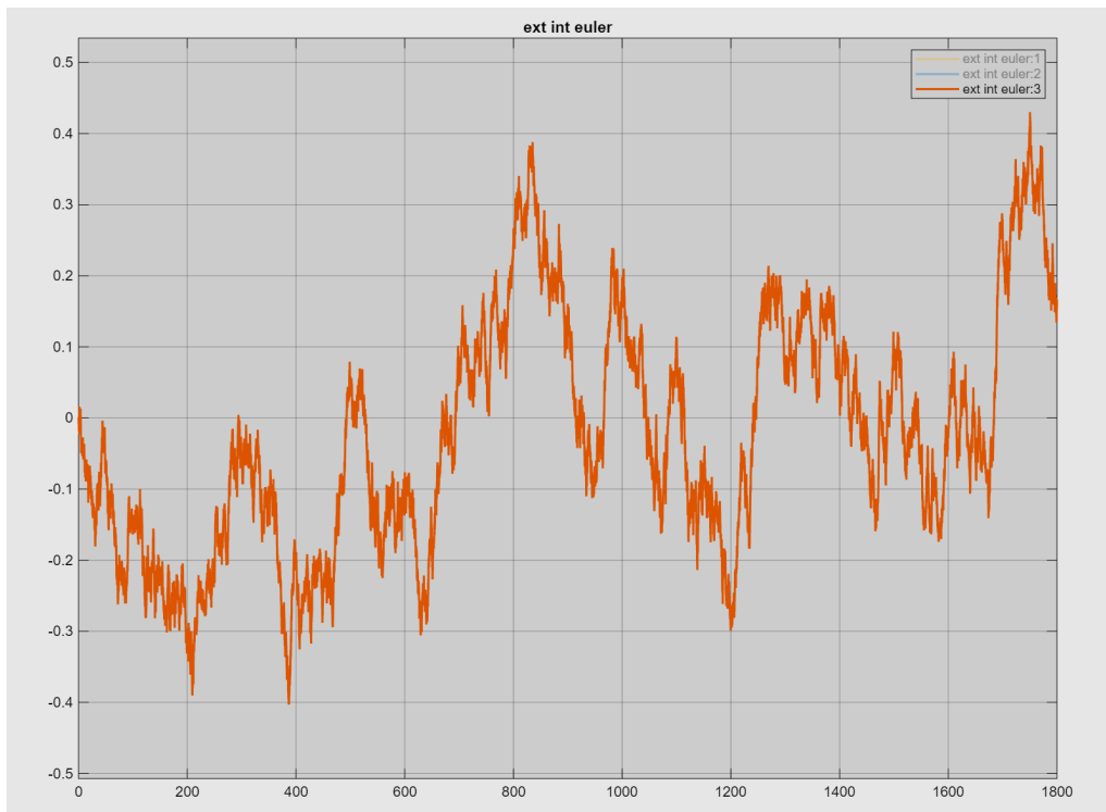
Figure 5.9: Time evolution of the altitude estimation error resulting from pure mechanization, with ESKF applied.
