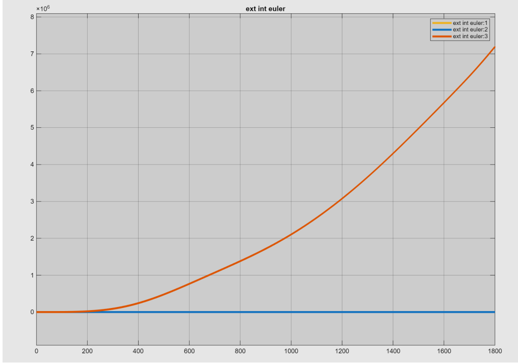
Figure 5.7: Time evolution of the position estimation error resulting from pure mechanization, with no filter applied.
