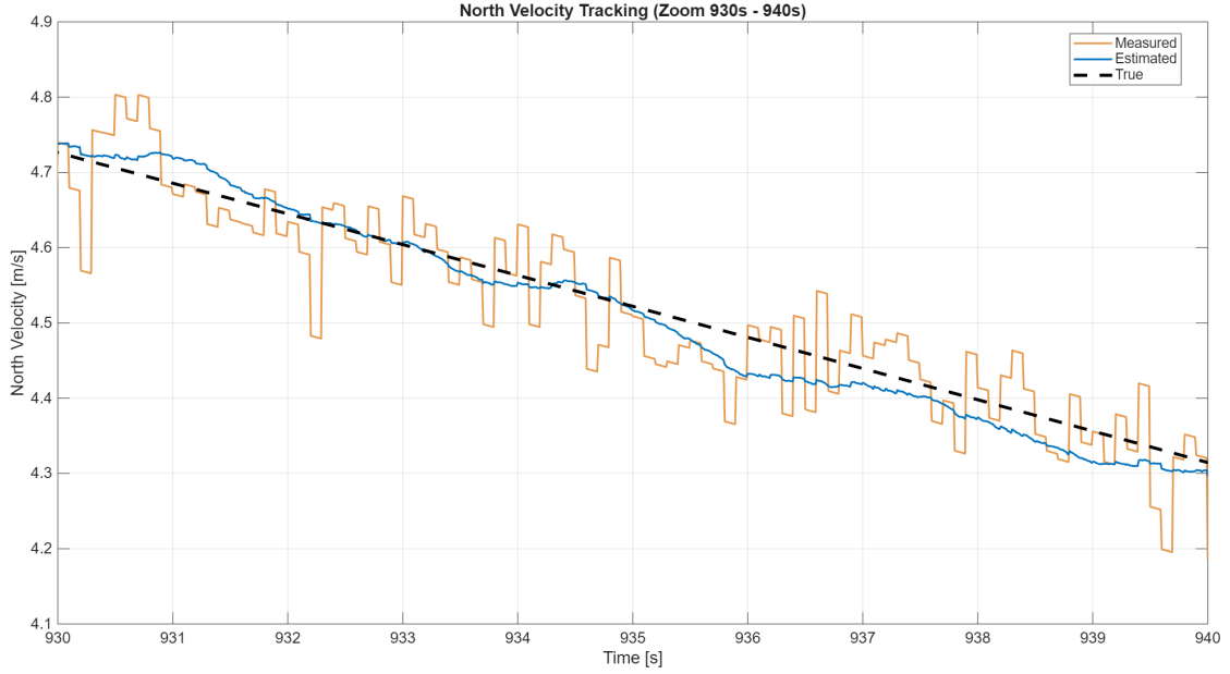
Figure 5.12: North velocity trajectory tracking (zoomed): Comparison between ground-truth, noisy GNSS measurement, and the ESKF estimation.
