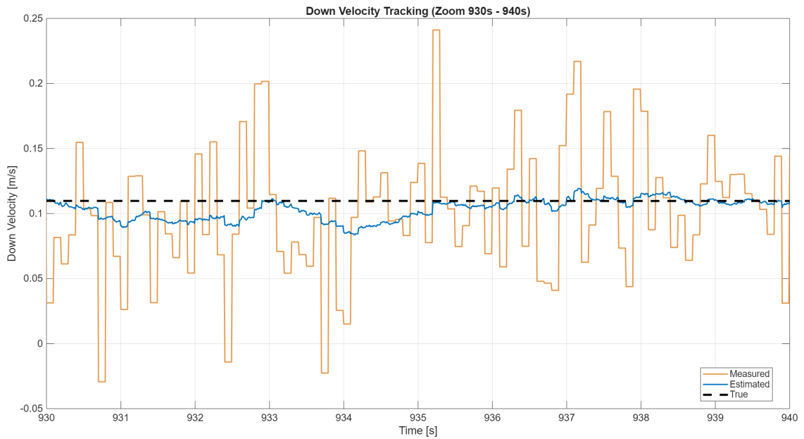
Figure 5.14: Down velocity trajectory tracking (zoomed): Comparison between ground-truth, noisy GNSS measurement, and the ESKF estimation.
