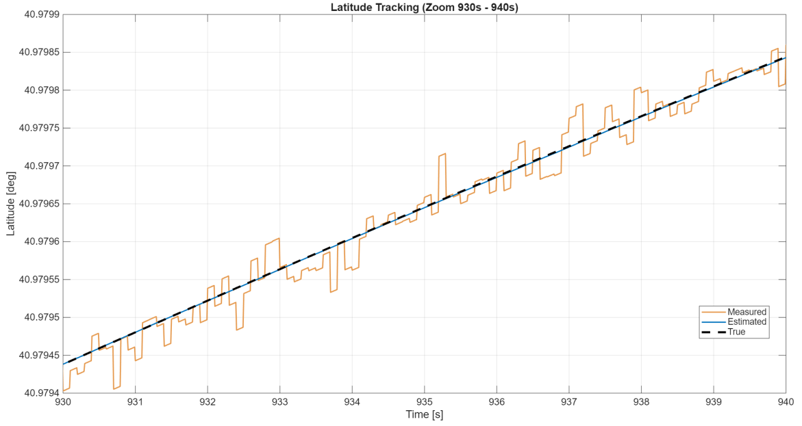
Figure 5.15: Latitude trajectory tracking (zoomed): Comparison between ground-truth, noisy GNSS measurement, and the ESKF estimation.
