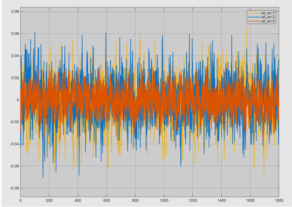
Figure 5.11: Time evolution of the velocity estimation error resulting from pure mechanization, with ESKF applied.
