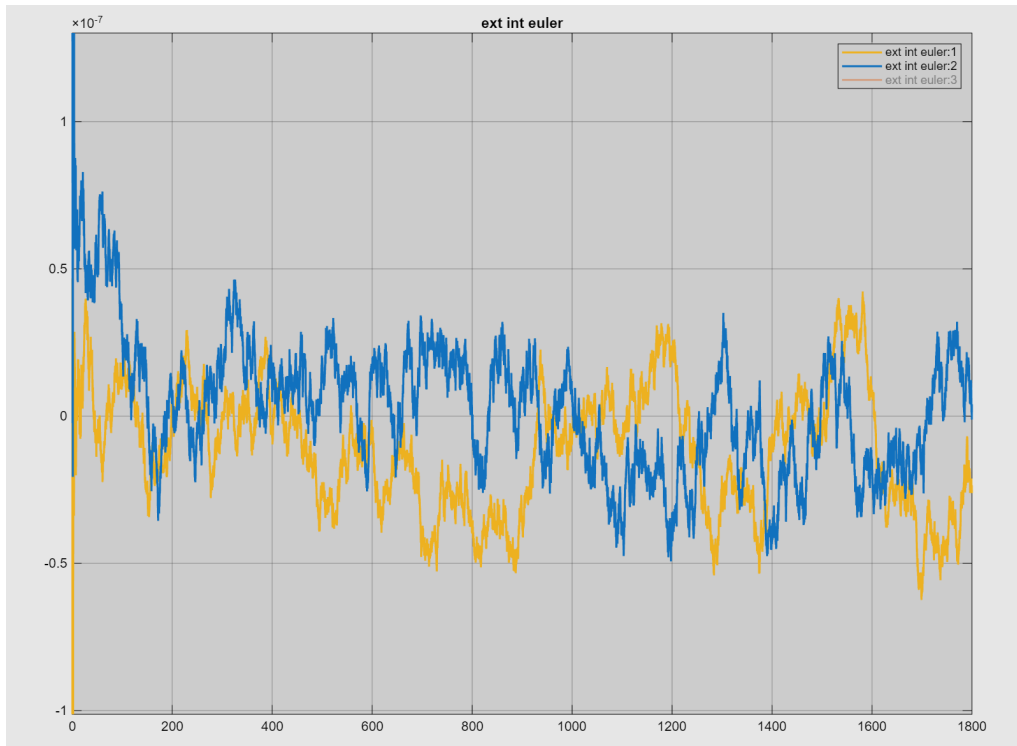
Figure 5.11: Time evolution of the latitude/longitude estimation error resulting from pure mechanization, with ESKF applied.
