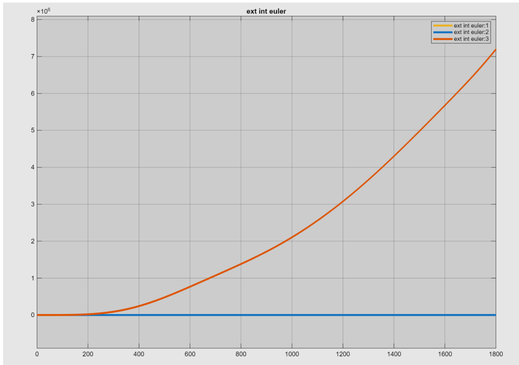
Figure 5.10: Time evolution of the position estimation error resulting from pure mechanization, with no filter applied.
