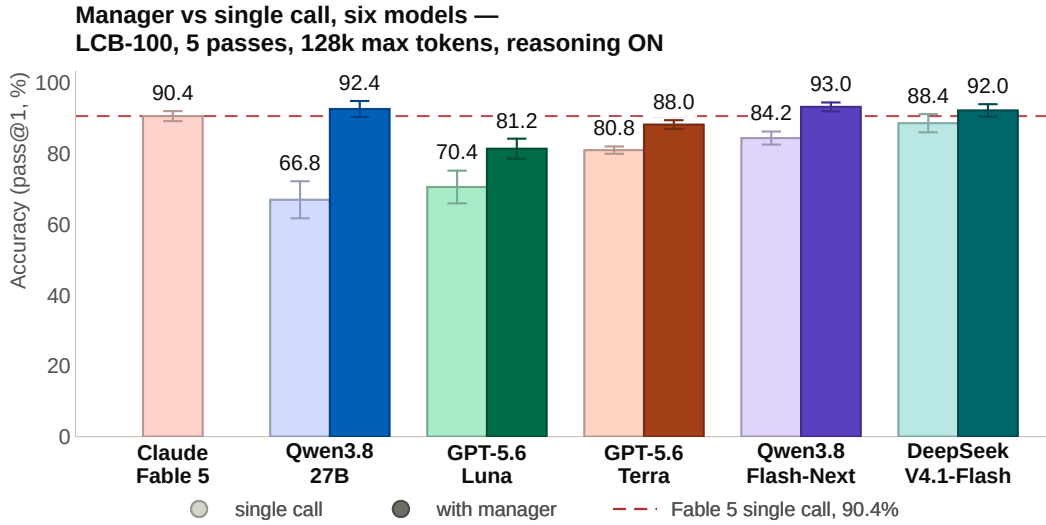
Figure 2: Manager vs. single call. The scores from Table 1 in a graph. Bars are pass@1 on the same 100 problems, the line through each the 95% CI across the 5 passes ( t , df = 4 ). The left bar of each pair is the single call, light; the manager is beside it, dark; colour is the model. Fable 5 ran single-only, so it has one bar, which the dashed rule carries across the chart.
