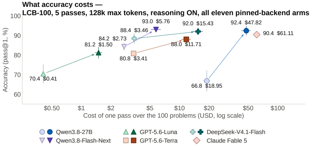
Figure 3: Cost against accuracy. One point per arm; an arrow runs from the single call to the manager of each model that has both. x is dollars for one pass over the 100 problems (log scale), y is pass@1; the bar through each point is the 95% CI across the 5 passes ( t , df = 4 ). Light fill = single call, dark = with manager; marker shape is the model.
