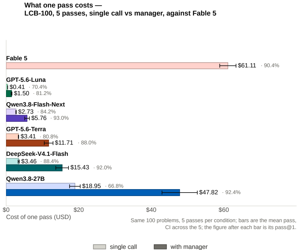
Figure 4: The scaffold’s bill. Cost of one pass over the same 100 problems; Table 2 is the arithmetic behind every bar. No cached-input discount is taken, and Qwen3.8-27B is priced at OpenRouter market rates. The top bar of each pair is the single call, light; the manager is under it, dark; all are at a 128k output cap, and colour is the model. Fable 5 is first; the models below it run top to bottom from the cheapest single call to the dearest. Table 2 carries the tests. Unbracketed comparisons: every manager – single increase is significant, and GPT-5.6-Luna’s manager undercuts GPT-5.6-Terra’s single call by $1.91. At 1.28x the assumed Qwen rate ($0.273/$3.26 per MTok, inside the spread across hosted providers) the manager’s cost advantage over Fable 5 disappears entirely — a larger uncertainty than any p-value here.
