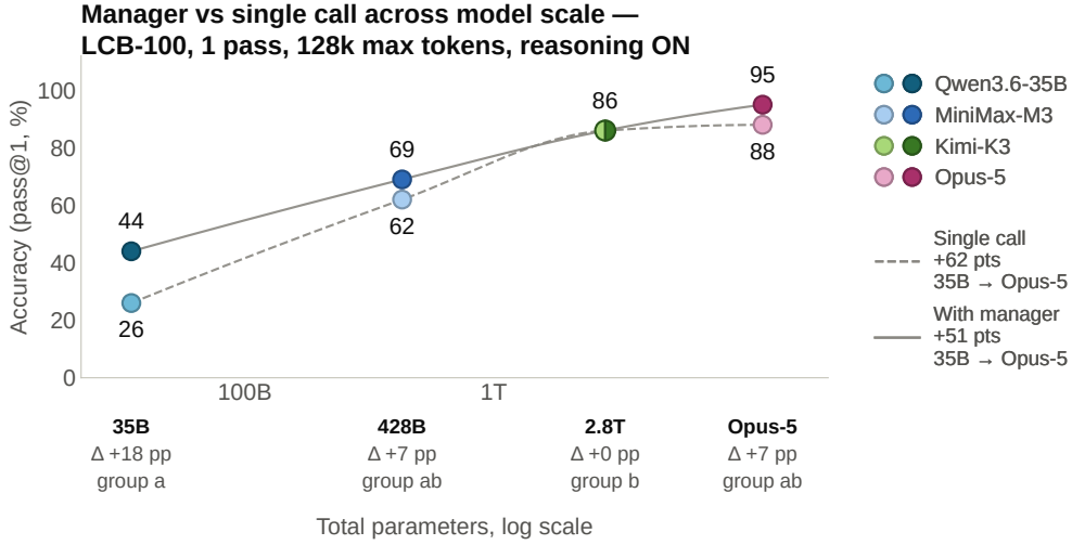
Figure 6: Accuracy by model scale, reasoning on, 128k, one pass. The same numbers as Figure 5a, against parameter count. Dashed = single call, solid = with manager; the block under each tick gives that model's \Delta and Tukey group, and the legend each arm's gain from the smallest model to the largest.
