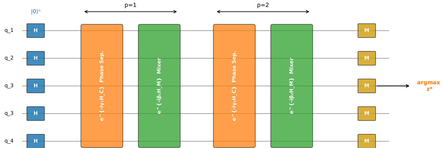
Figure 2: QAOA Circuit for Node Selection QUBO cost: c_n = \beta_1 T^{\xi_k}(\alpha, n) + \beta_2 E^{\xi_k}(\alpha, n)
