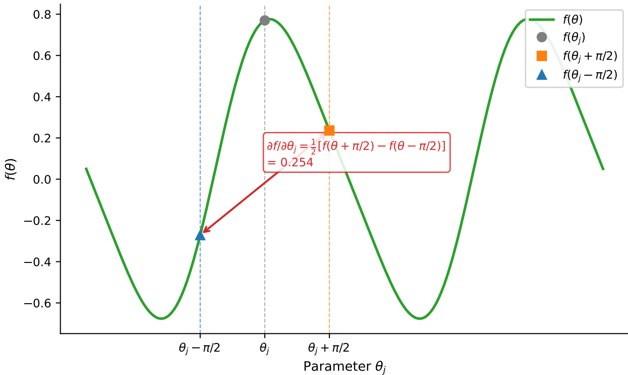
Figure 3: Parameter Shift Rule for VQC Gradient Estimation
