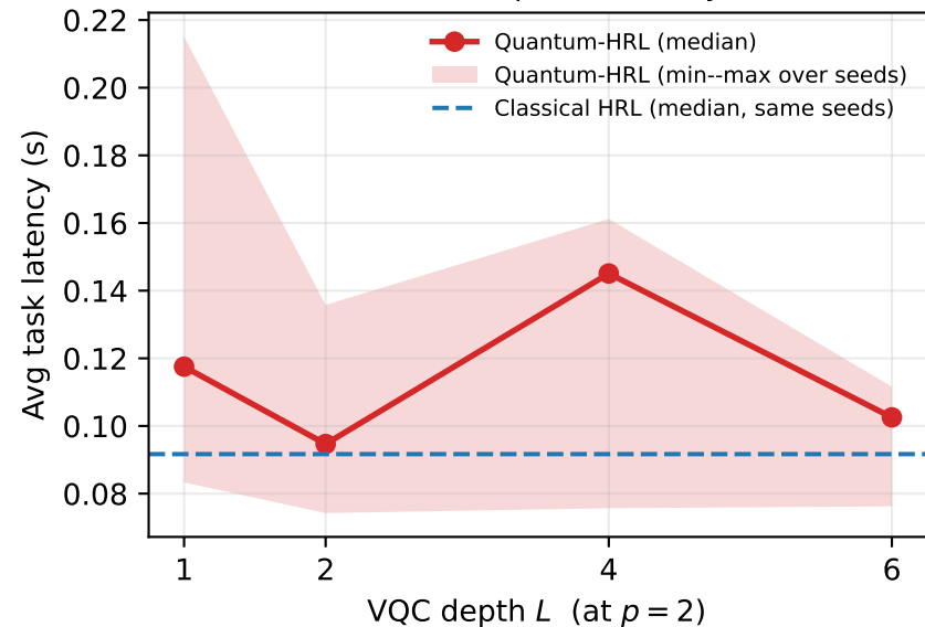
(a) VQC depth sensitivity
