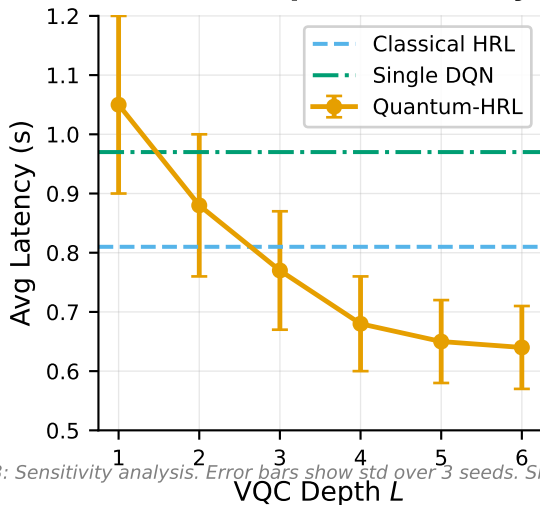
(a) VQC Depth Sensitivity
