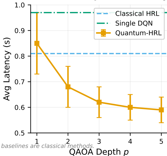
(b) QAOA Depth Sensitivity
