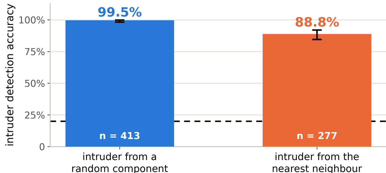
Components are coherent without their labels
