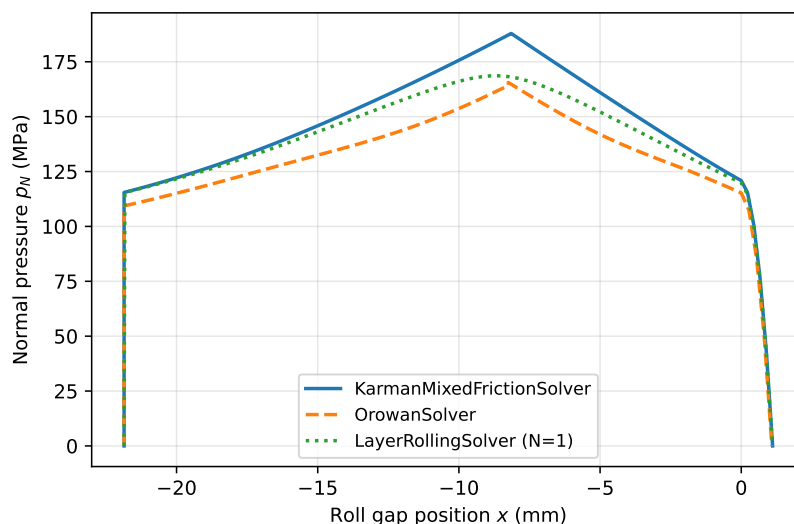
Figure 4: Normal-pressure distribution across the roll gap for the same pass as Table 3, comparing KarmanMixedFrictionSolver , OrowanSolver and LayerRollingSolver ( N = 1 ).
