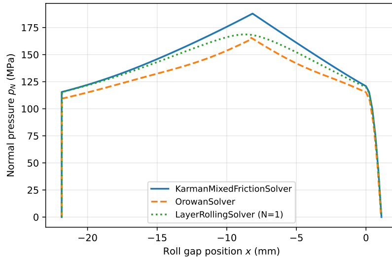
Figure 5: Normal-pressure distribution across the roll gap for the same pass as Table 3, comparing KarmanMixedFrictionSolver , OrowanSolver and LayerRollingSolver ( N = 1 ).
