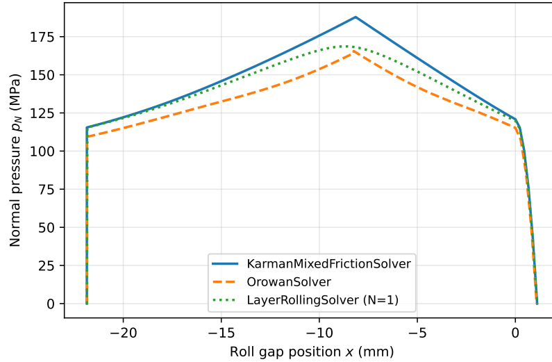
Figure 2: Normal-pressure distribution across the roll gap for the same pass as Table 3, comparing KarmanMixedFrictionSolver , OrowanSolver and LayerRollingSolver ( N = 1 ).
