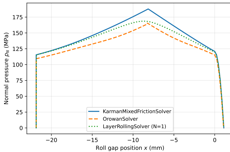
Figure 3: Normal-pressure distribution across the roll gap for the same pass as Table 3, comparing KarmanMixedFrictionSolver , OrowanSolver and LayerRollingSolver ( N = 1 ).
