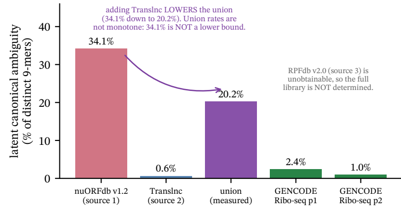
(a) Libraries differ enormously — and do NOT compose
