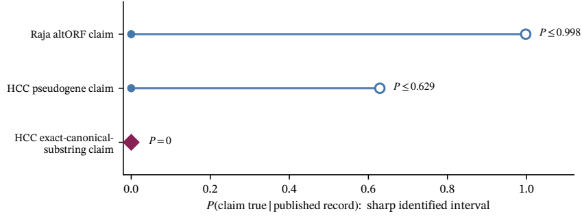
FIGURE 4. Per-claim truth is a partial order. For a claim not yet individually inspected beyond class membership, truth admits only a sharp class-conditioned upper bound on P(\text{true}) , not a point value: a random Raja altORF claim P \leq 0.998 , a random HCC pseudogene claim P \leq 0.629 . Once a claim’s own status is observed that value collapses to a point instead: an exact-canonical-substring claim has P = 0 , regardless of class. Both non-degenerate intervals share the lower bound 0, so the class-conditioned case is an upper-bound ranking, not set-dominance. Intervals are drawn open-capped at the upper bound (a bound, not a confirmed value); the filled diamond marks the point-identified P = 0 case.
