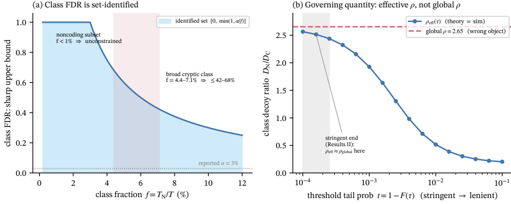
FIGURE 3. The identifiability theory. (a) The class-specific FDR is only set-identified; the sharp upper bound is \min(1, \alpha/f) , giving \leq 42-68\% for the broad cryptic class ( f = 4.4-7.1\% ) at the reported \alpha = 3\% . (b) A diagnostic: the class decoy split follows a threshold-weighted effective \rho , not the global candidate ratio: simulated D_N/D_C tracks \rho_{\text{eff}}(\tau) and drifts from \rho_{\text{global}} as the threshold relaxes; the shaded band marks this simulation’s stringent end, where \rho_{\text{eff}} \approx \rho_{\text{global}} — the limit Results II characterizes as typical for immunopeptidomics operating conditions, without establishing that any given cohort actually sits there.
