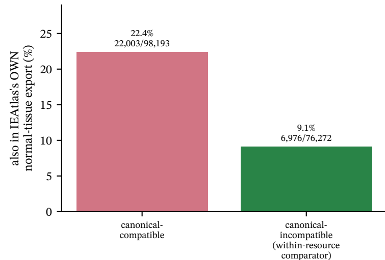
(a) Adjusted risk ratio 1.72\times [1.66, 1.80]
