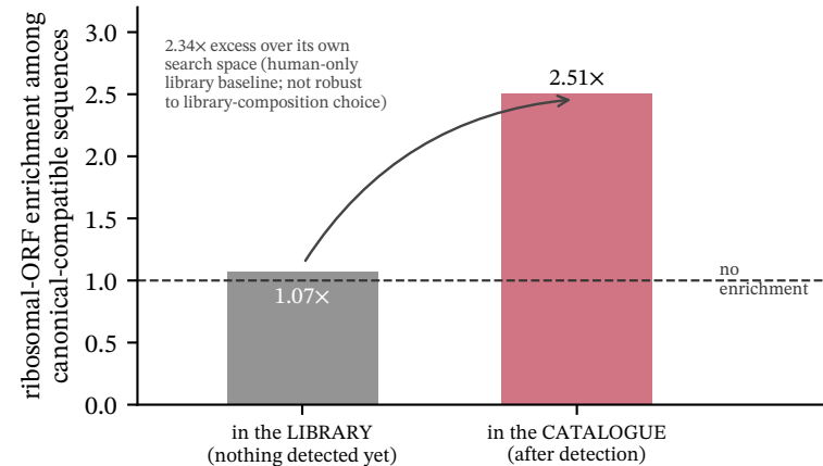
(a) The library does not account for the catalogue's enrichment
