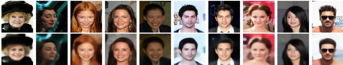
FIGURE 15 – Reconstitution test
