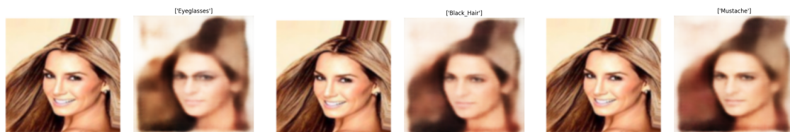
FIGURE 16 – Ajout lunettes
