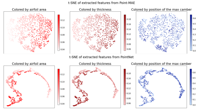
Fig. 3. t-SNE visualization of the latent spaces. Each point represents one airfoil, and its position corresponds to the global feature vector extracted by the pretrained model. The colors indicate known geometric properties that were meaningful for airfoil geometries: airfoil area, thickness, and the position of the maximum camber.
