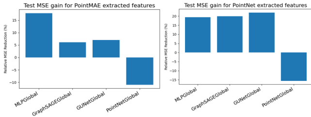
Fig. 8. Impact of the extracted features on the surrogate models performances
