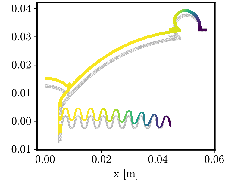
Mode 1 115.1 Hz \zeta=0.029
