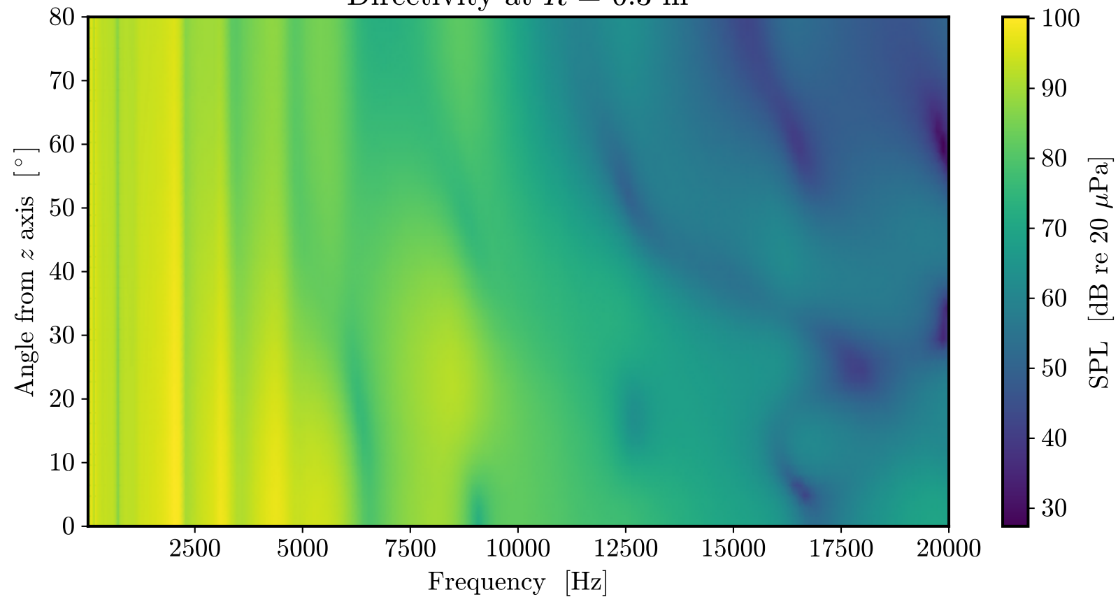
Directivity at R = 0.3 m
