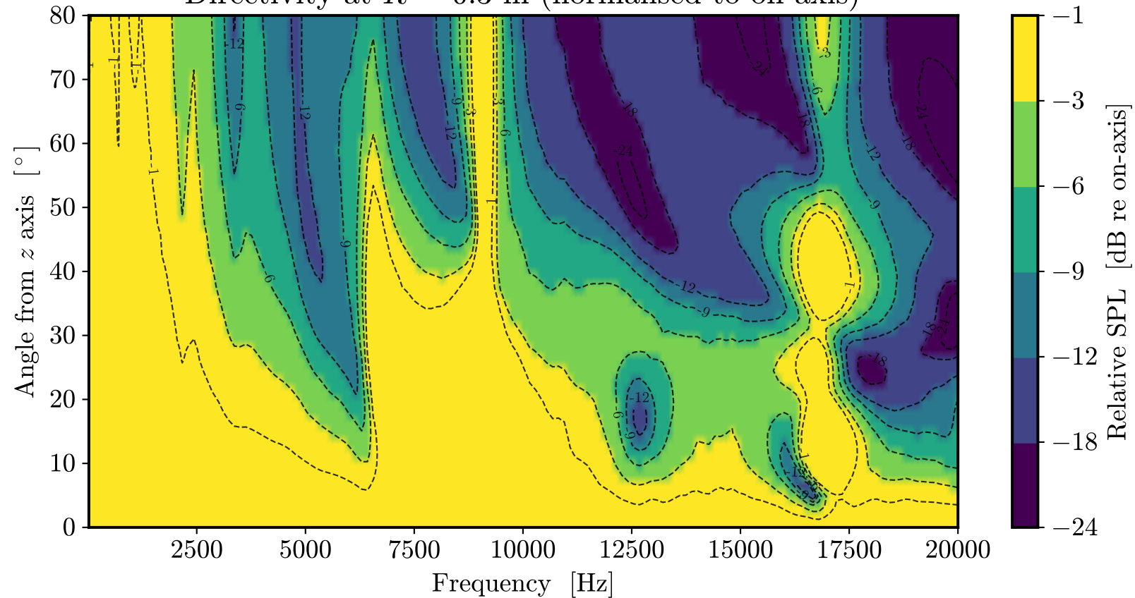
Directivity at R = 0.3 m (normalised to on-axis)
