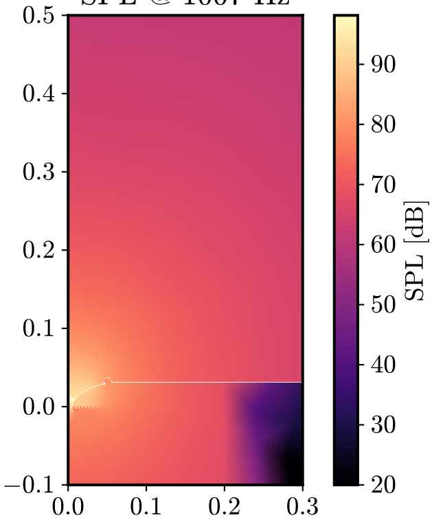
SPL @ 1007 Hz
