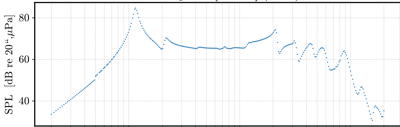
SPL at probe [0.3 0.1] (front)
