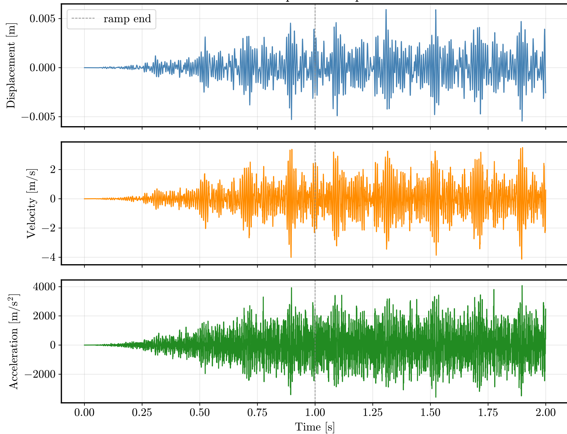
Cone tip - time response
