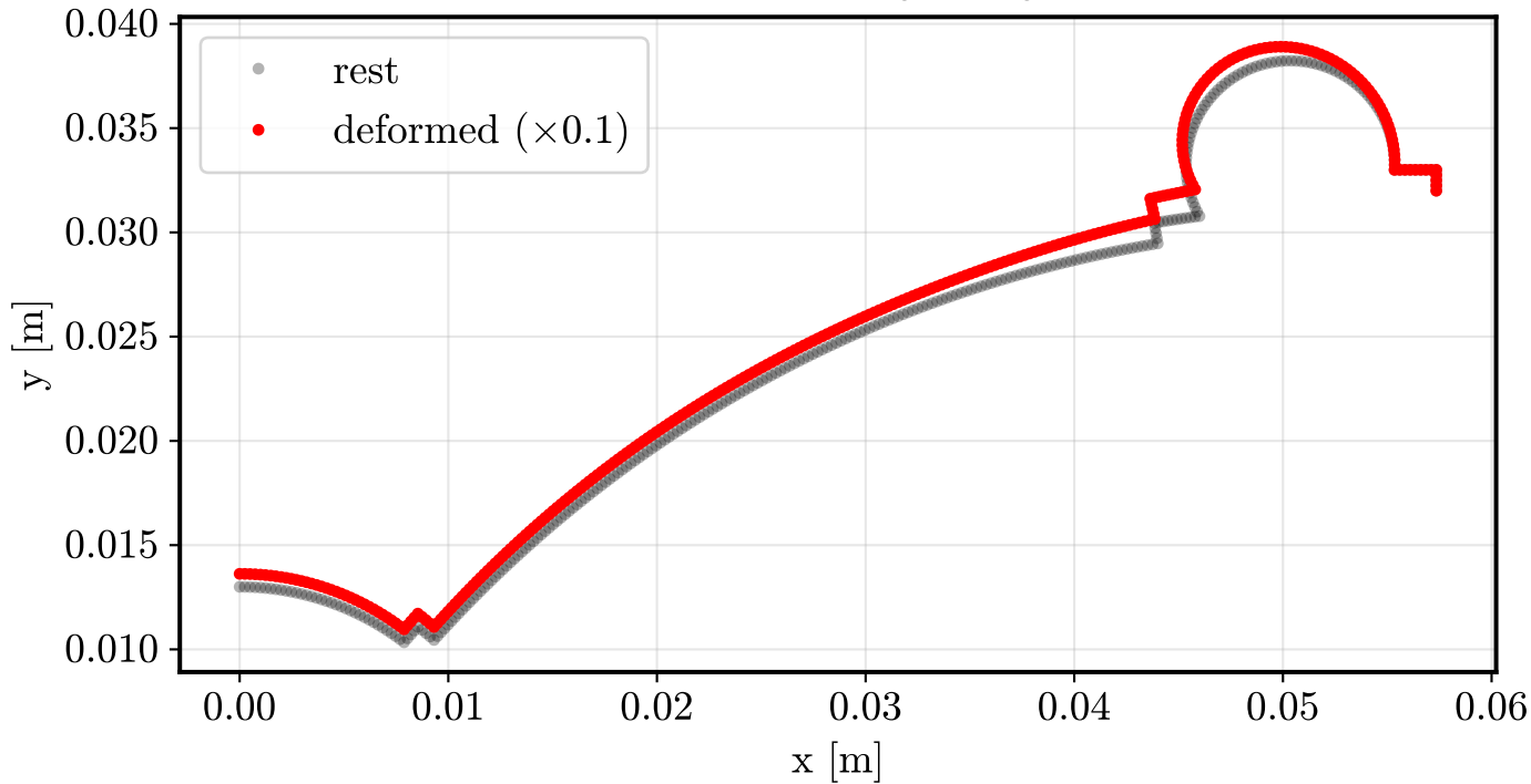
Interface - mode 3 - 419.2 Hz
