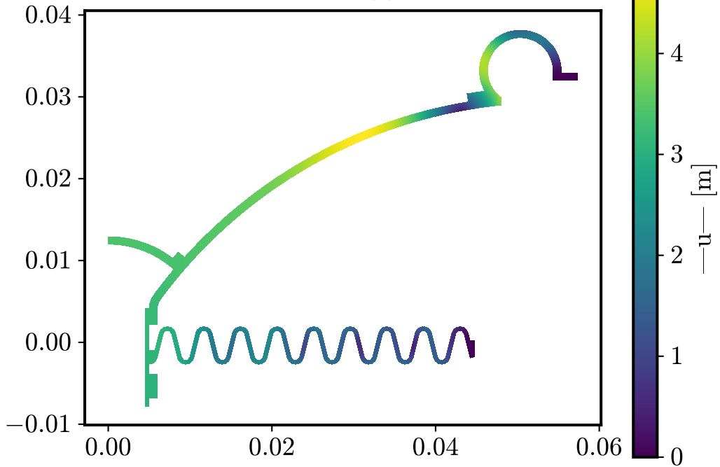
—u— @ 1001 Hz
