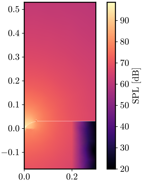
SPL @ 1001 Hz
