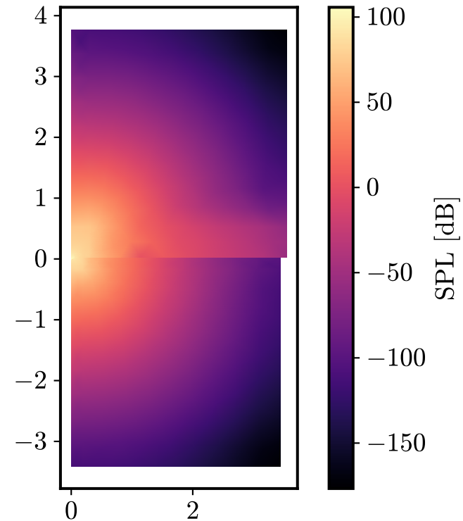
SPL @ 106 Hz
