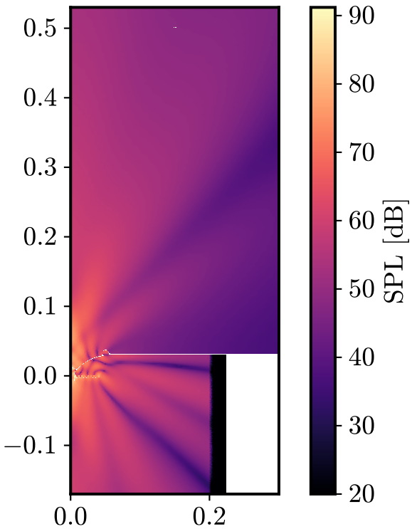
SPL @ 14394 Hz
