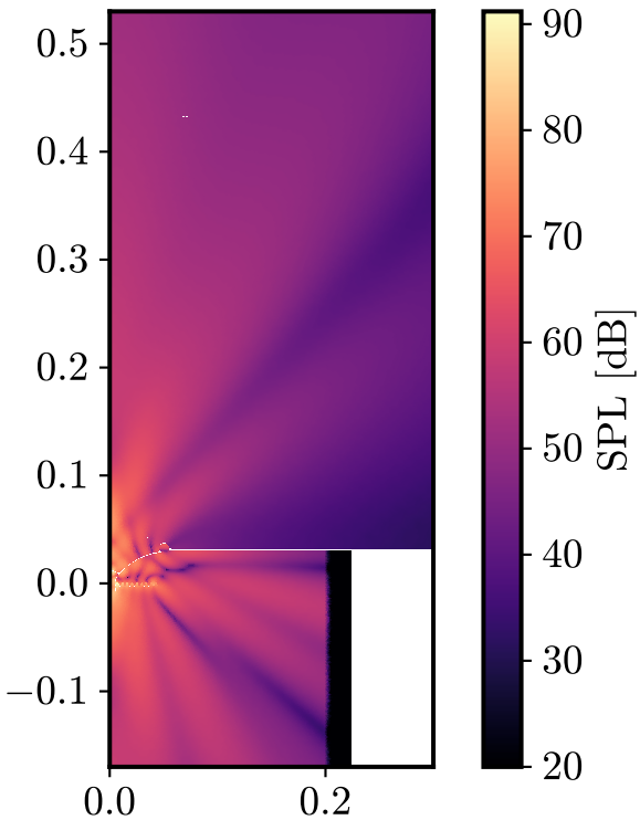
SPL @ 14901 Hz
