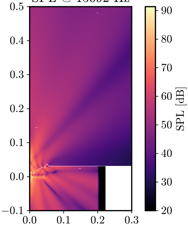
SPL @ 15092 Hz
