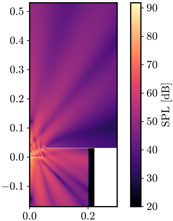
SPL @ 15761 Hz
