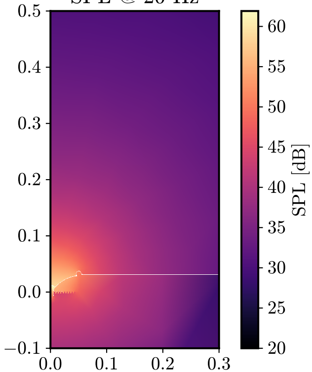
SPL @ 20 Hz
