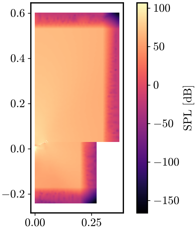
SPL @ 4790 Hz
