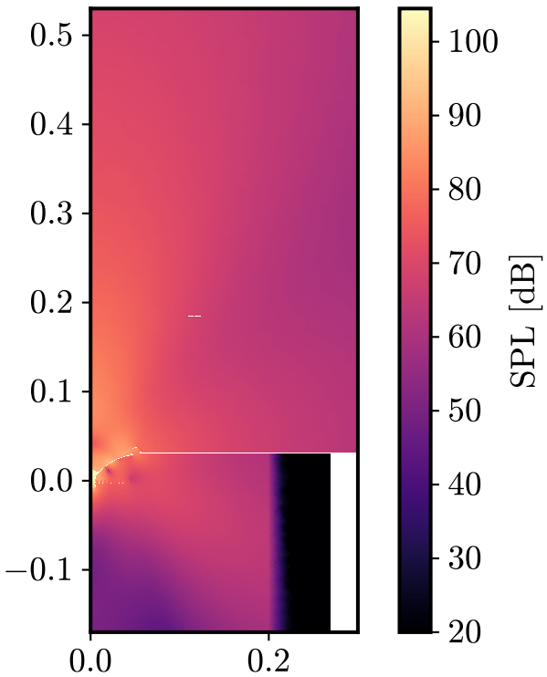
SPL @ 5006 Hz
