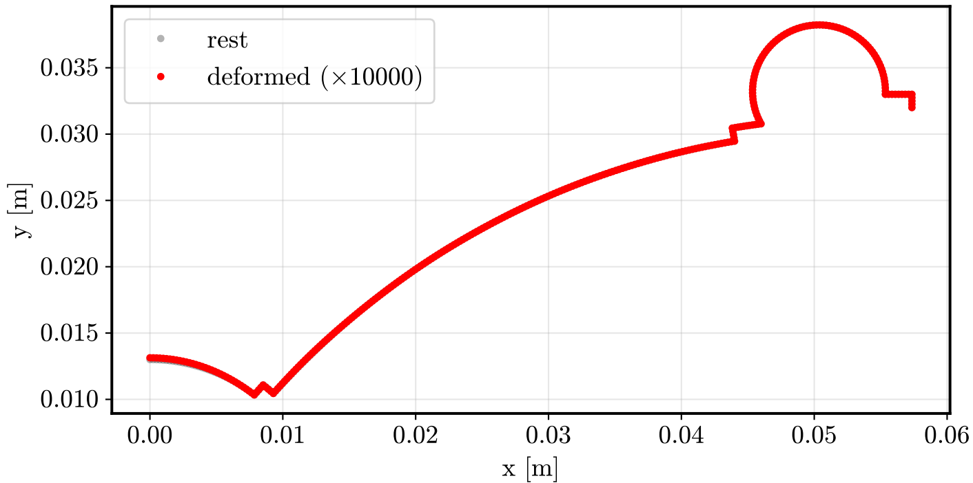
Interface deformation @ 14394 Hz
