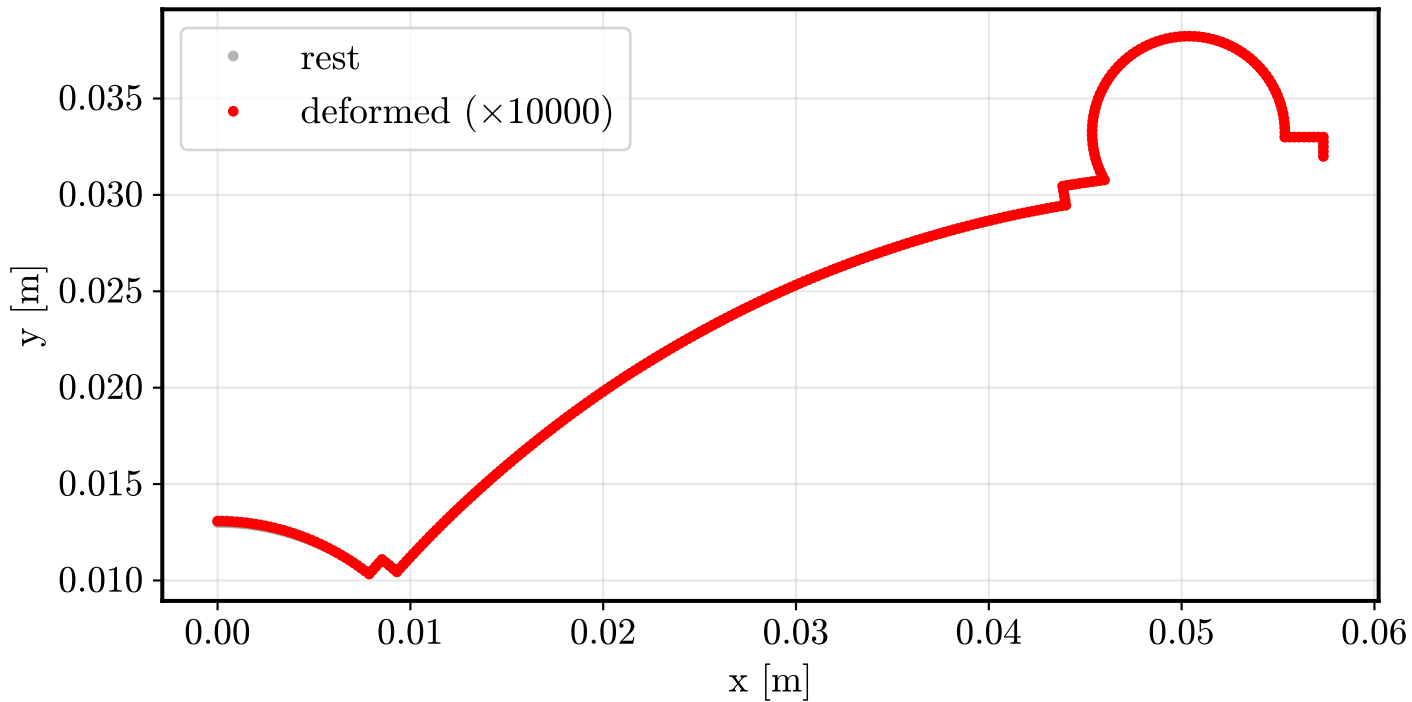
Interface deformation @ 15761 Hz
