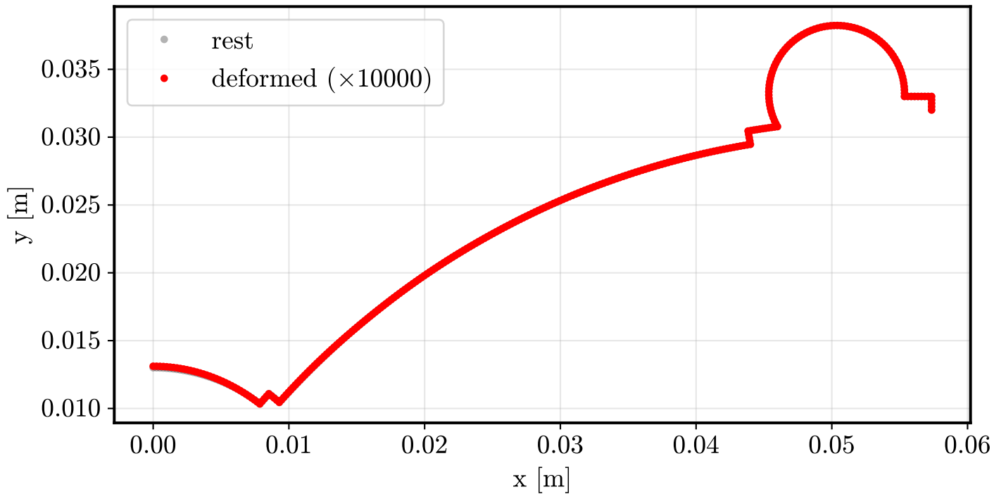
Interface deformation @ 14901 Hz
