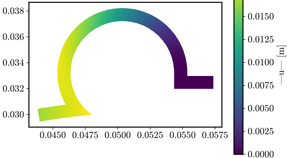
Surround - mode 3 - 419.2 Hz
