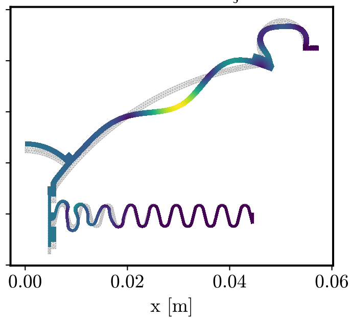
Mode 21 3257.6 Hz \zeta=0.0537
