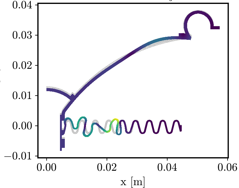
Mode 17 2155.4 Hz \zeta=0.0342
