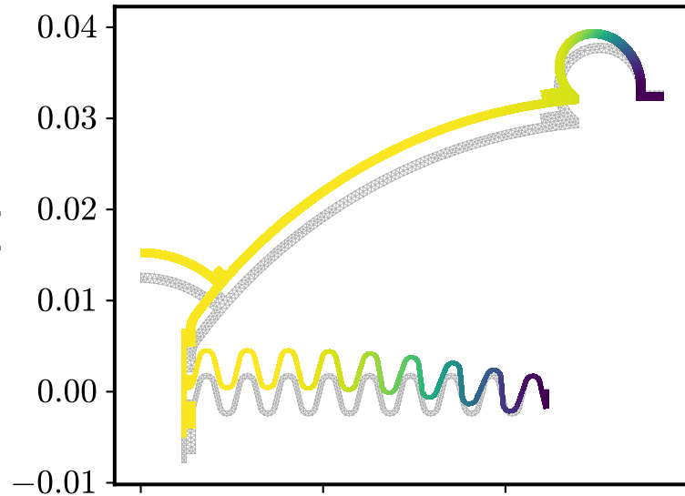
Mode 1 115.1 Hz \zeta=0.0393
