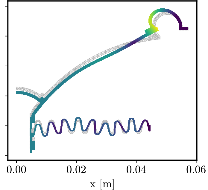
Mode 5 733.2 Hz \zeta=0.0244
