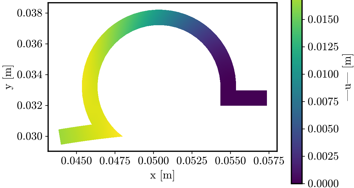
Surround - mode 3 - 419.2 Hz
