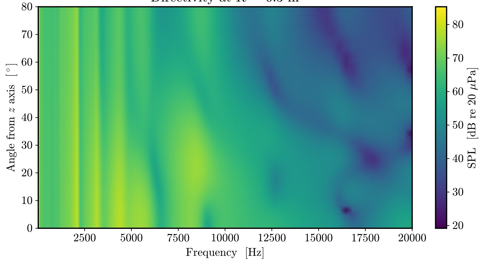
Directivity at R = 0.3 m
