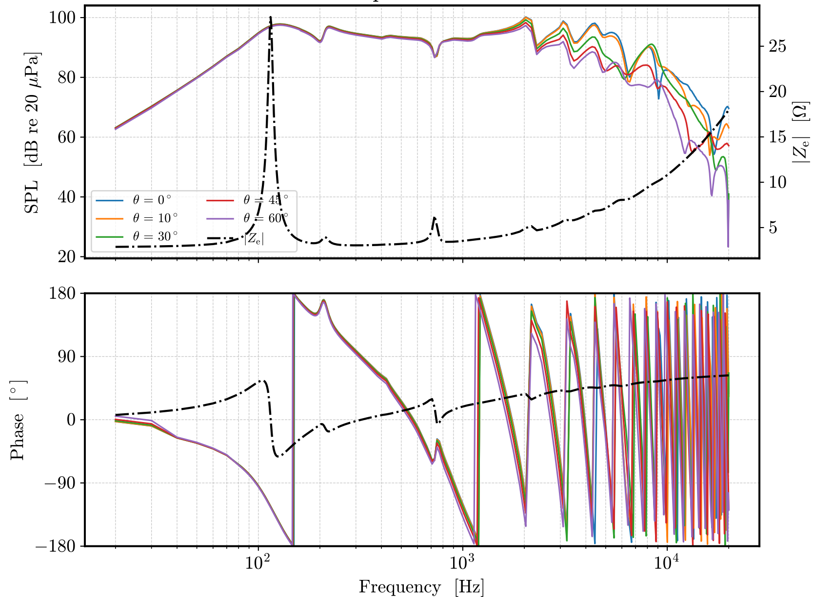
SPL and phase at R = 0.3 m
